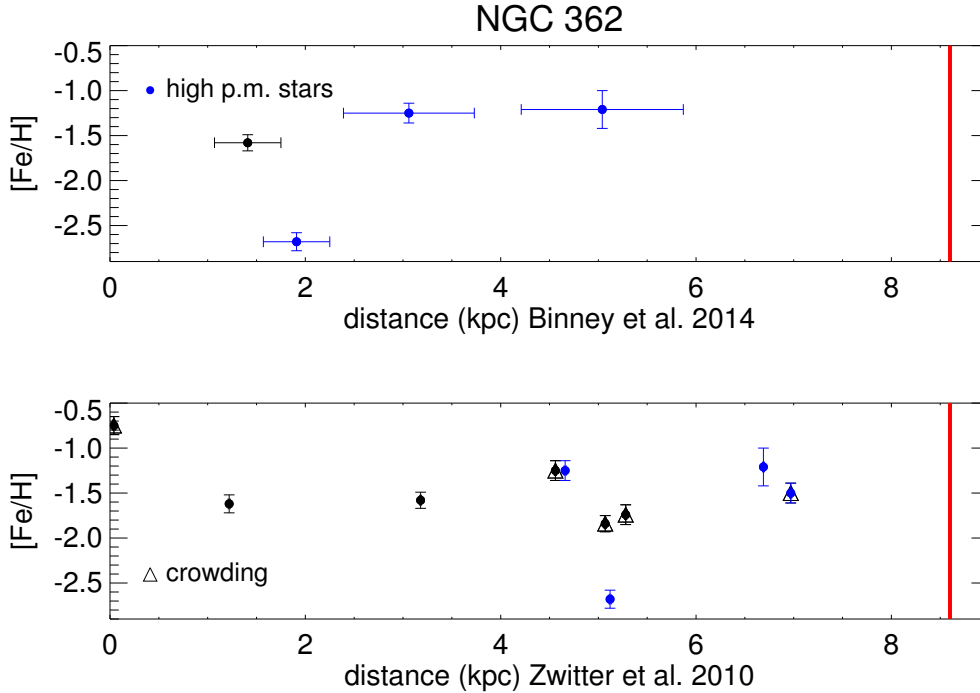
Figure 18. Distance vs. [Fe/H] for the members of NGC 362. In the top panel are plotted the distances derived in Binney et al. (2014); however, there are only 4 stars with this information. In the bottom panel the distances from Zwitter et al. (2010) are shown. Blue dots are stars with a large proper motion; triangles indicate stars affected by crowding. The vertical red line indicates the distance of the cluster from Harris (1996) (2010 edition).
