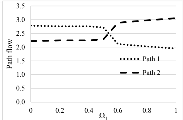
Figure 3(b). Path flows
