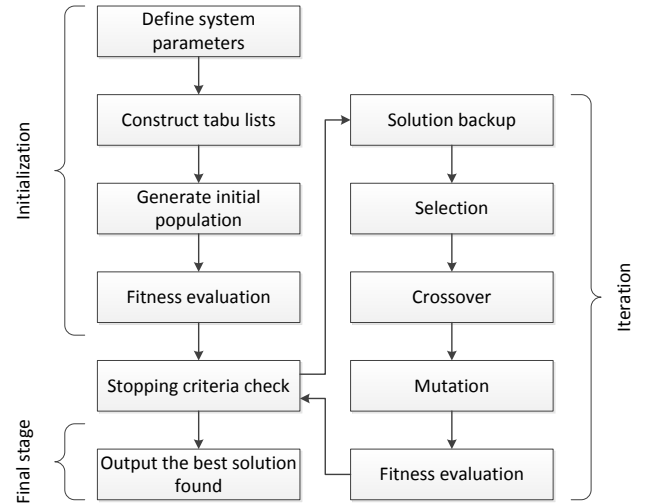
Fig. 4. Flow chart of the algorithm.
