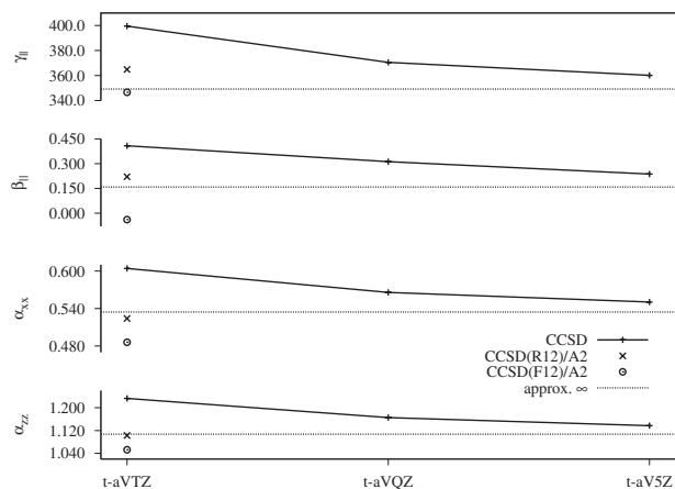
FIG. 5. Basis set convergence of the electronic correlation contributions to static polarizabilities \alpha_{zz} and \alpha_{xx} and first and second hyperpolarizabilities \beta_{\parallel} and \gamma_{\parallel} for CO (in a.u.) using the t-aVXZ basis sets with triply augmented diffuse functions. A2 stands for ansatz 2.
