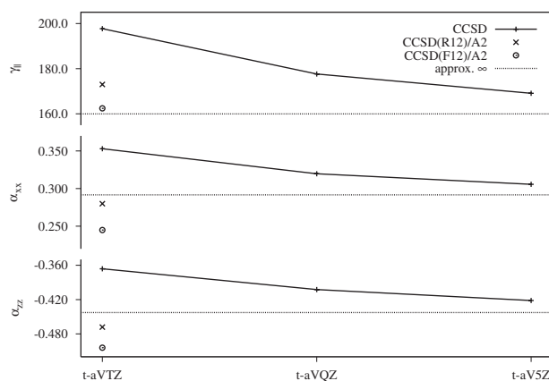
FIG. 6. Basis set convergence of the electronic correlation contributions to static polarizabilities \alpha_{zz} and \alpha_{xx} and second hyperpolarizabilities \gamma_{\parallel} for N_2 atom (in a.u.) using the t-aVXZ basis sets with triply augmented diffuse functions. A2 stands for ansatz 2.
