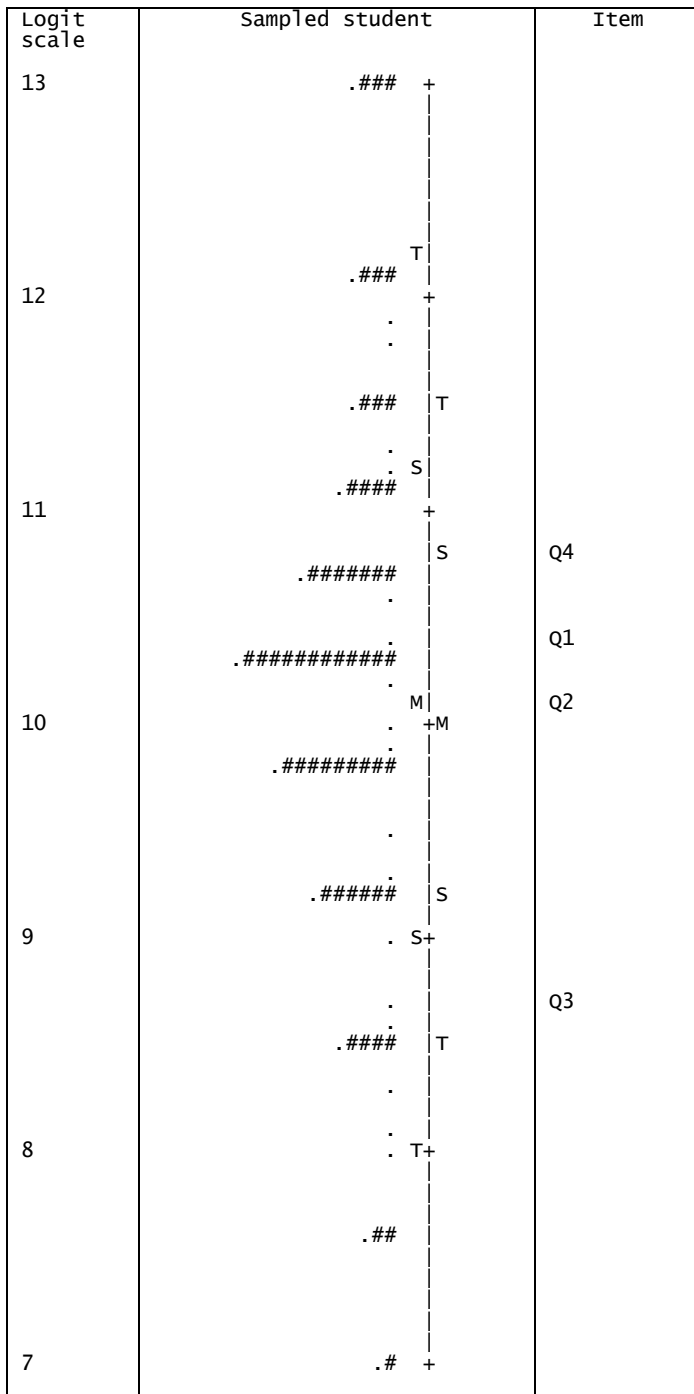
Figure 1. Person-Item Map (The first column is the logit scale for the item and person Rasch measures. The second and third columns are the distributions of students and items, respectively. Each '#' represents 47 students and each '.' represents 1-46 students. The 'M' on the left and right represent the mean for person estimates and the mean for item estimates, respectively. 'S' represents one sample deviation away from the mean, and 'T' represents two sample deviations away from the mean. From the map, it can be seen that most of the students stayed within one sample standard deviation from the mean.)
