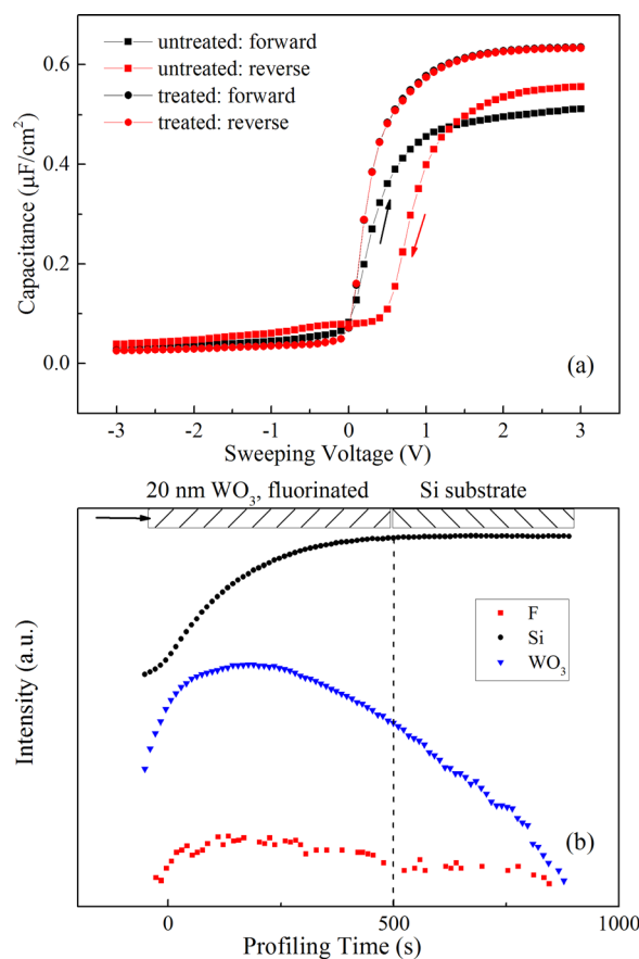
FIG. 2. (a) Capacitance-voltage characteristics of the \text{WO}_3 based capacitors. (b) SIMS profile of the fluorine-plasma-treated \text{WO}_3 deposited on Si substrate.
