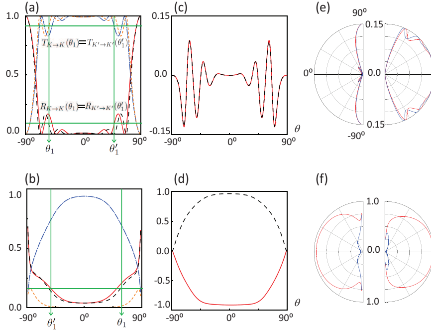
FIG. 2: (color online) (a) and (b): Reflection coefficients R_{K' \rightarrow K}(\theta) (red solid lines), R_{K \rightarrow K}(\theta) (black long-dashed lines) and transmission coefficients T_{K' \rightarrow K}(\theta) (blue dash-dot lines), T_{K \rightarrow K}(\theta) (orange short-dashed lines). (c) and (d): The valley fluxes j_v^R(\theta) (the red solid line) and j_v^T(\theta) (the black long-dashed line), illustrating valley filters (as (c)) and valley sources (as (d)). (e) and (f): The out-going angle distributions of the reflected (the left semi-circle) and the transmitted (the right semi-circle) fluxes carrying valley K (the blue line) and K' (the red line). (a), (c) and (e) are in filter-dominating regime with U_g = -77.4\text{meV} while (b), (d) and (f) are in the source-dominating regime, using U_g = -530\text{meV} . In (a), the intersects between the green vertical and horizontal lines exemplifies the equality shown on the plot's vicinity. These equalities underlie the cancellation of opposite valley fluxes by time-reversal paired scattering events. In (b), only R_{K \rightarrow K}(\theta_1) = R_{K' \rightarrow K'}(\theta'_1) is identified. The lack of such equality in transmission coefficients signifies the importance of inter-valley scattering. The incident energy E_{\text{in}} is measured from conduction band bottom, E_F , by E_{\text{in}} - E_F = 44.24\text{meV} . Other well shape parameters are S = 10a and W = 110a , where a is the lattice constant. These parameters are fixed otherwise specified. The slight asymmetry between \theta'_1 and \theta_1 with respect to 0^\circ is due to the trigonal warping of the fermi contours.
