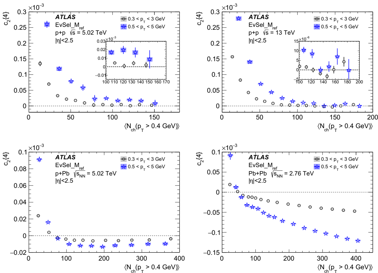
Fig. 7 Comparison of c_2\{4\} obtained for two p_T ranges of reference tracks as a function of \langle N_{ch}(p_T > 0.4 \text{ GeV}) \rangle for 5.02 TeV and 13 TeV p+p collisions, and 5.02 TeV p + \text{Pb} collisions, and 2.76 TeV \text{Pb} + \text{Pb} col-
