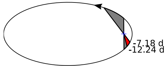
Figure 1. Upper panel: The r_s and r_{BH} as function of \phi . The red curves are r_s corresponding to different n , and the dashed black curve is r_{BH} . \phi is the true anomaly and the zero point is at the periastron. In both panels \rho_0 = 1 \times 10^{-9} \text{ g/cm}^3 . Bottom panel: The illustration of the orbit and the position of the disk (grey shade region). The arrow indicates the sense of motion of the pulsar. The red shade is the region where mass transfer takes place when n = 3.3 . The number beside the orbit is the days after periastron of the start and end of the mass transfer.
