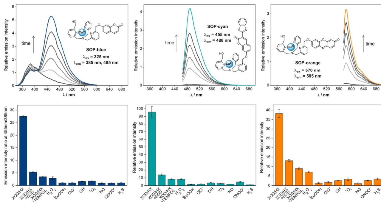
Fig. 1. (a) Time-dependent fluorescence response (0, 3, 5, 7, 10, 60 min) of 5 \mu M SOP-blue (left), SOP-cyan (center) and SOP-orange (right) towards superoxide (xanthine oxidase: 10 mU/ml; hypoxanthine: 75 \mu M); and (b) selectivity towards 20 eq. of other reactive species. Error bars are \pm SD ( n = 3 ).
