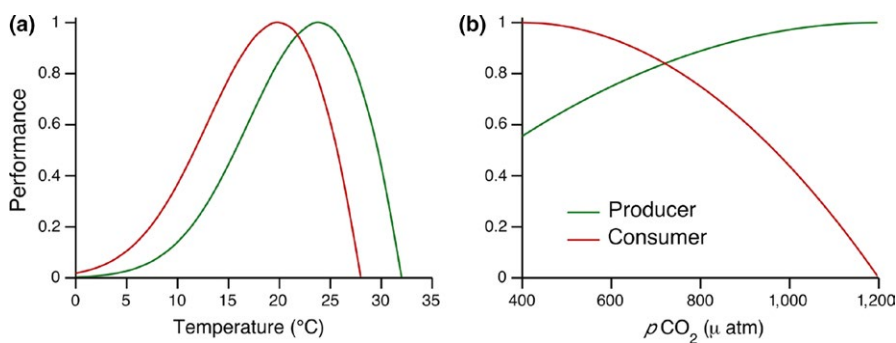
FIGURE 2 Species vary in their physiological responses to abiotic factors such as (a) temperature and (b) pCO 2 . Green lines indicate a hypothetical primary producer, and red lines represent a hypothetical consumer. When such relationships differ among interacting species, relative performance levels change with absolute value of the environmental driver
