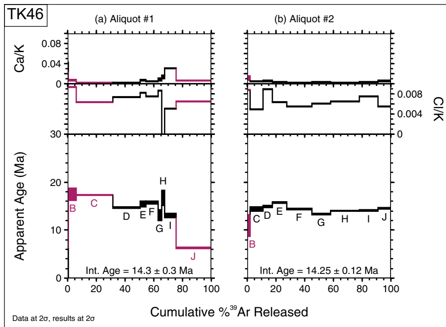
Figure 9. White mica step-heating plots for TK15 and TK46. All data and results are presented at 2σ. All aliquots run for each specimen are shown. Each step is labeled as corresponds to data in Supplemental Table 4 (footnote 5). Integrated (Int.) ages are reported for each aliquot. For TK46, the integrated ages reported in the plots were calculated using only the steps in black (i.e., red steps were excluded) and reflect the dominant 40 Ar/ 39 Ar age group (see text for discussion).
