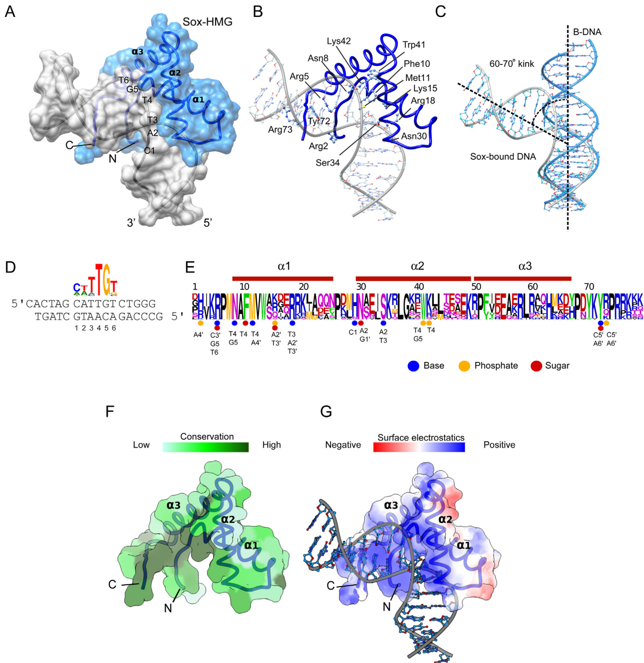
Fig. 1. DNA recognition by the Sox HMG box.
