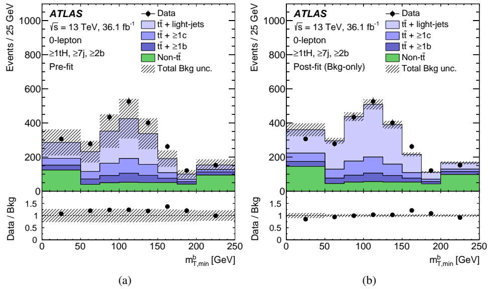
Figure 16: Comparison between the data and prediction for the distribution of the minimum transverse mass of E_T^{\text{miss}} and any of the three leading b -tagged jets in the event ( m_{T,\text{min}}^b ) in the ( \geq 1tH , \geq 7j , \geq 2b ) region of the 0-lepton channel (a) before and (b) after performing the combined fit of the m_{\text{eff}} spectrum to data in the 0-lepton and 1-lepton channels search regions (“Pre-fit” and “Post-fit”, respectively) under the background-only hypothesis. The small contributions from t\bar{t}V , t\bar{t}H , single-top, W/Z +jets, diboson, and multijet backgrounds are combined into a single background source referred to as “Non- t\bar{t} ”. The last bin in all figures contains the overflow. The bottom panels display the ratios of data to the total background prediction (“Bkg”). The hashed area represents the total uncertainty of the background. In the case of the pre-fit background uncertainty, the normalisation uncertainty of the t\bar{t} + \geq 1b background is not included.
