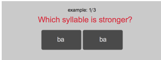
Figure 2: Experiment interface.
