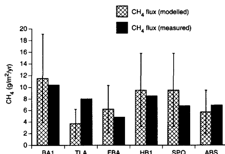
Fig. 3. Modelled and measured annual methane emission estimates at various northern wetland sites. The error bars on model values represent the range given the \text{CH}_4/\text{CO}_2 ratio. BA1: Bethel, Alaska, 61°N, 162°W (Bartlett et al., 1992; Fan et al., 1992). TLA: Toolik Lake, Alaska, 68°N, 149°W (Christensen, 1993). FBA: Fairbanks, Alaska, 64°N, 145°W (Whalen and Reeburgh, 1992). HB1: Hudson Bay Lowlands, 51°N, 81°W (Moore et al., 1994; Roulet et al., 1994). SPQ: Schefferville, Quebec, 55°N, 66°W (Moore et al., 1990). ABS: Abisko, Sweden, 68°N, 20°W (Svensson and Roswall, 1984).
