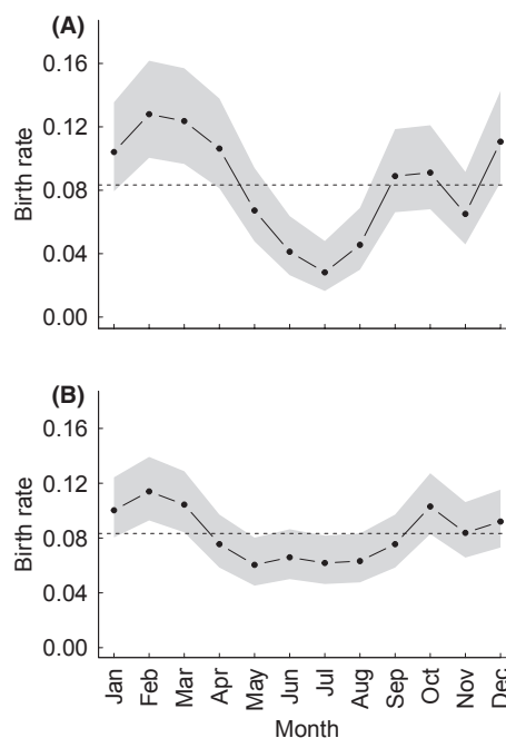
Figure 3. Predictions of monthly probability of birth-by-birth order in Asian elephants from Myanmar. (A) Firstborn calves ( n = 893 ) and (B) later-born calves ( n = 1457 ). Points indicate the predicted probability from the model and shaded area represents the 95% confidence interval on parameter estimates. The dashed line indicates the predicted birth rate if births were distributed evenly across months. Predictions are for males (similar pattern is observed in females).
