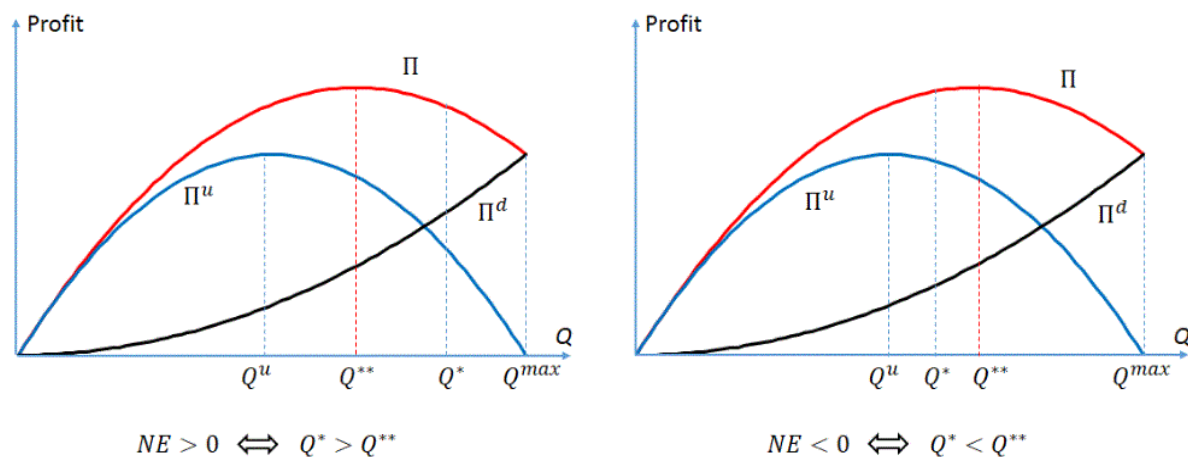
Figure 1: Profit curves as functions of Q
