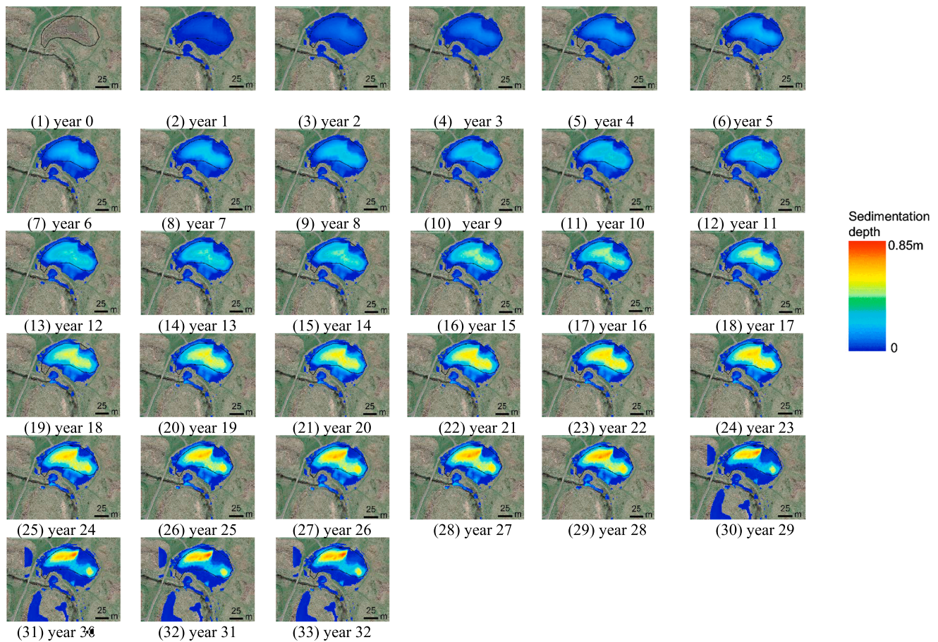
Fig. 11. Cumulative annual sediment deposition from 1984 to 2015.
