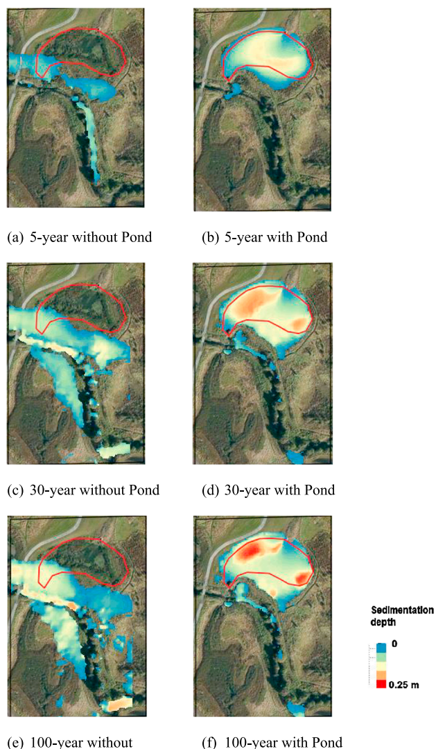
Fig. 10. Sediment deposition for 5-year, 30-year, 100-year events for 'with' and 'without' pond scenarios.
