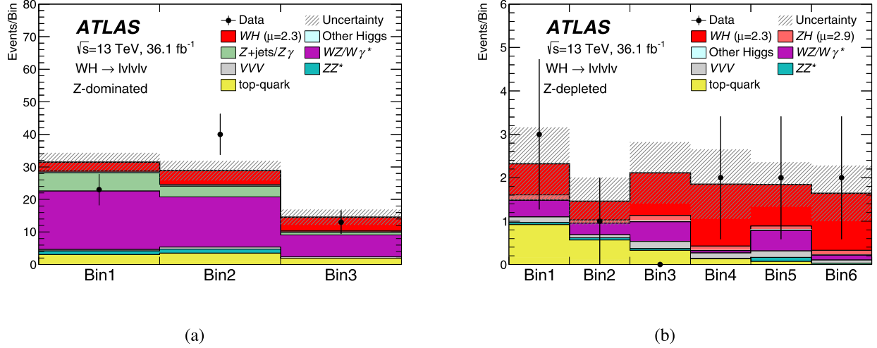
Fig. 6. Post-fit BDT-score distributions (a) in the WH Z-dominated SR and (b) for the two-dimensional grid in BDT_{\tilde{t}\bar{t}} and BDT_{WZ} in the WH Z-depleted SR. The shaded band includes statistical and systematic uncertainties on both signal and background as estimated by the fit.
