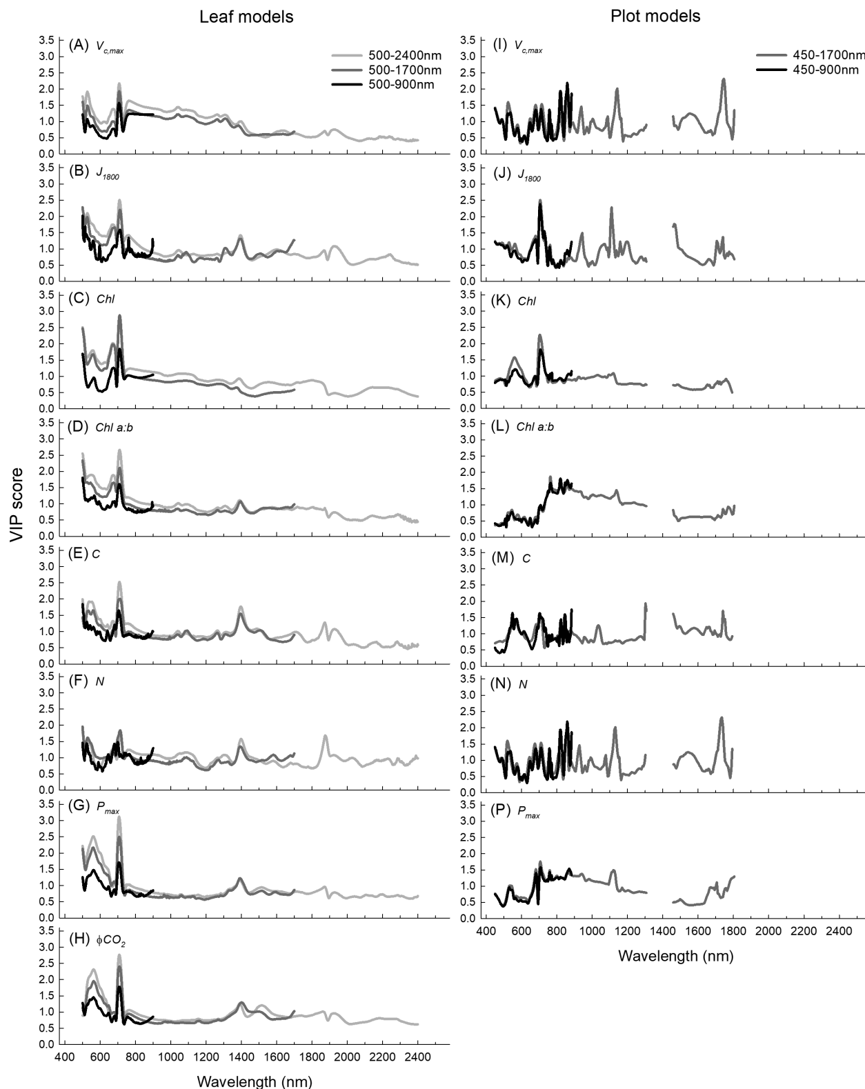
Fig. 8. PLSR model variable importance projection (VIP) scores for models built with different spectral ranges for leaf level and for V_{c,max} (A), J_{1800} (B), chlorophyll content (C), Chl\ a:b (D), C content (E), N content (F), P_{max} (G), and \phi CO_2 (H), and at the plot level for the same traits, respectively (I–P). VIP scores for plot-level \phi CO_2 models are not shown due to the lack of predictability of this parameter at the plot level.
