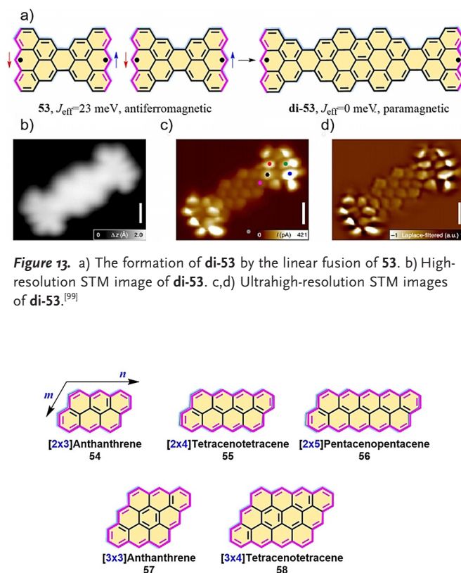
Figure 14. Chemical structures of the rhombus nanographenes.
