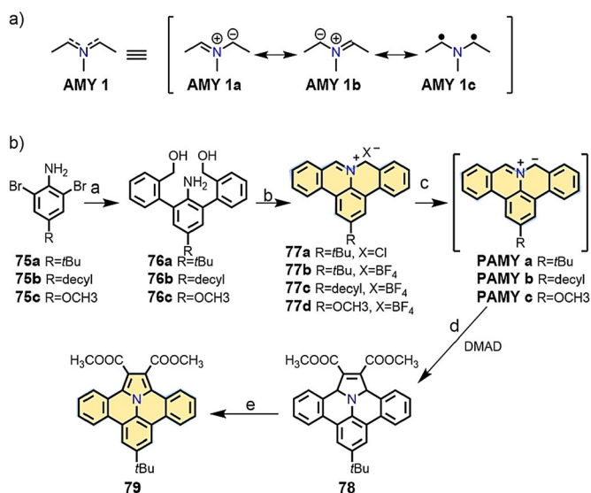
Scheme 9. a) The resonance structures of AMY 1 . b) Synthesis of 79 . [116]
