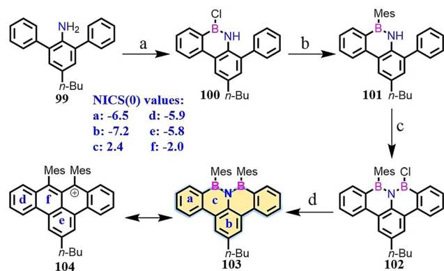
Scheme 14. Synthesis of BNB-edged 103 with mesityl groups. [126]
