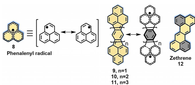
Figure 4. Phenalenyl radical ( 8 ) and its resonance forms, biphenalenyls 9–11 and their resonance forms, and zethrene ( 12 ).
