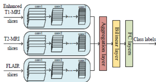
Figure 6. A 2D convolutional network in combination with the multimodal information fusion of MRI for the grading of brain-tumour gliomas (from [31]).
