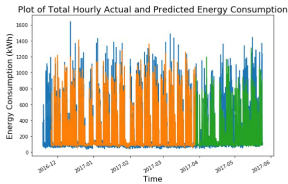
Figure 8. Plots of the actual versus predicted hourly energy consumption for a specific floor of a smart-building application using a deep-learning network (from [2]).
