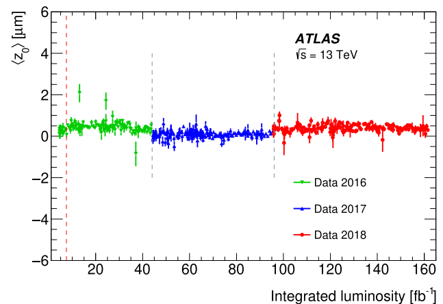
Fig. 24 The transverse (left) and longitudinal (right) impact parameter biases as function of the Run 2 delivered luminosity. The red dotted line indicate the change in the underlying ATLAS ID alignment geometry description. This splits the 2016 data in two periods. The grey dotted lines indicate the change of the data-taking years. The \sim 4 \text{ fb}^{-1} corresponding to 2015 data are not shown in this plot. Only statistical uncertainties are shown
