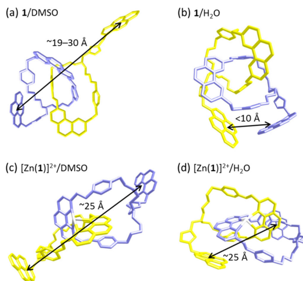
Fig. 3. Representative structures of 1 in (a) DMSO and (b) water, and [Zn(1)]^{2+} in (c) DMSO and (d) water obtained using MD simulations.
