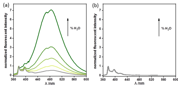
Fig. 2. Normalised emission spectra of a 25 \mu\text{M} solution of (a) 1 (unlocked state) and (b) [\text{Zn}(\mathbf{1})]^{2+} (locked state) in DMSO of increasing amount of water (0%, 60%, 70%, 80% and 90%).
