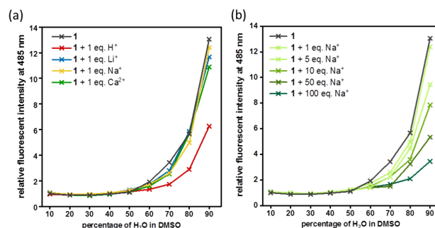
Fig. 4. Relative emission intensity at 485 nm of 1 in the presence of (a) 1 eq. of various cations and (b) increasing amount of Na^+ in DMSO of increasing amount of water (10% to 90%).
