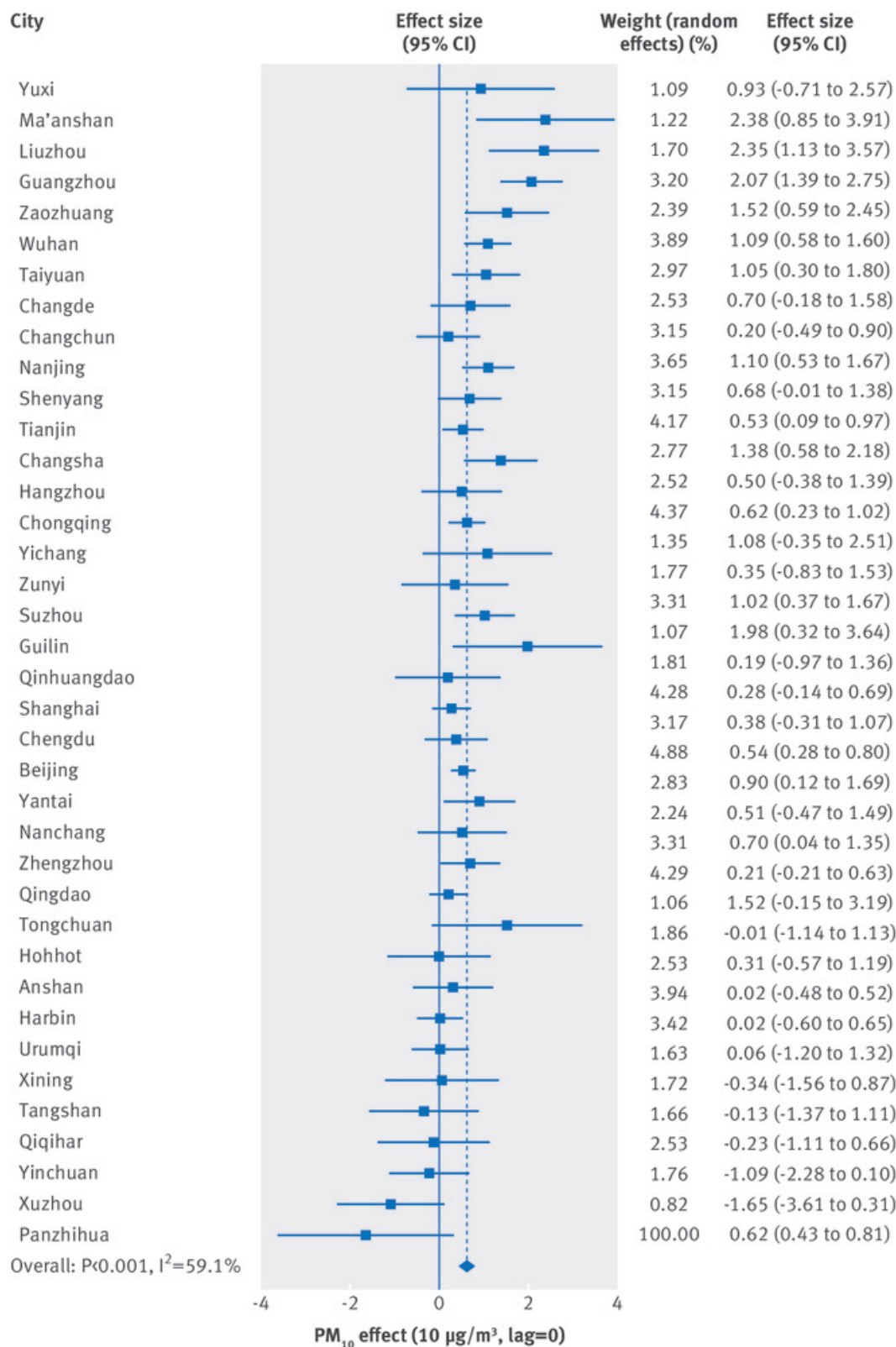
Fig 4 Maximum likelihood estimates (percentage) and 95% confidence intervals of the impact of 10 µg/m 3 PM 10 (lag=0) on total mortality for deaths due to cardiorespiratory diseases in 38 large cities in China. The dependent variable is the percentage change in number of daily deaths due to cardiorespiratory diseases. Each solid square represents an effect size. Horizontal lines indicate 95% confidence intervals
