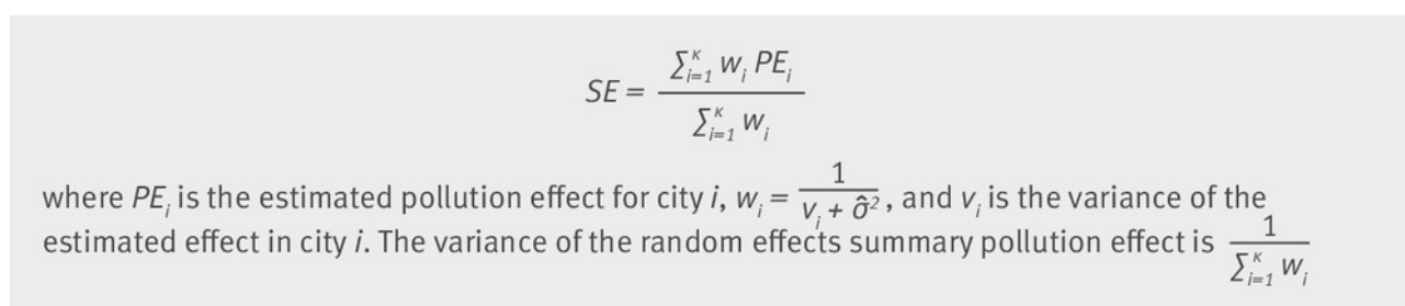
Fig 2 DerSimonian and Laird random effects summary estimate
