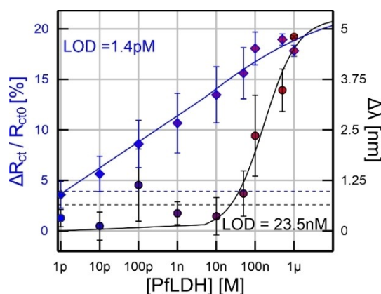
Figure 4. Calibration curves obtained for PflDH detection by simultaneously performed EIS (blue) and SPP (black) measurements with the hAu-based electrode aptasensor.
