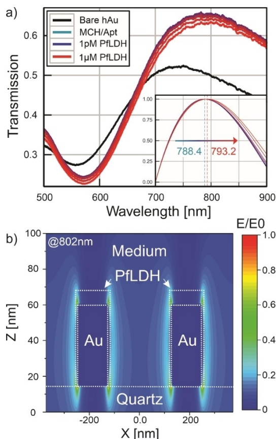
Figure 3. a) Transmission spectra of a bare gold nanohole arrays in air (black) and with different concentrations of PflDH (1 pM–1 \mu M) (blue-red) in buffer medium solution. The inset shows the zoom of normalized and fit transmission spectra at the surface plasmon polariton resonance revealing a red peak shift from 788.4 nm to 793.2 nm. b) FDTD simulated electrical field in the x-z cross-section of hAu electrode in the buffer medium.
