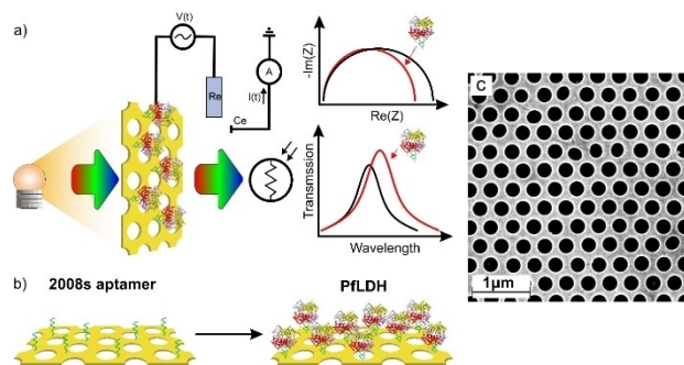
Figure 1. a) Sketch representing the dual aptasensor working principle. EIS and SPP detection are recorded from the gold nanohole array (hAu) electrode synchronously providing Nyquist plots of measured sample impedance and SPP transmission spectra. b) hAu aptasensor with immobilized aptamers and subsequent PfLDH detection. c) SEM image of hAu electrode with a lattice constant of 372 nm and a hole diameter of 245 nm.
