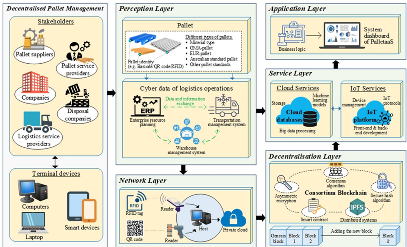
Figure 2. Layered architecture of PalletaaS for the decentralised pallet management.
