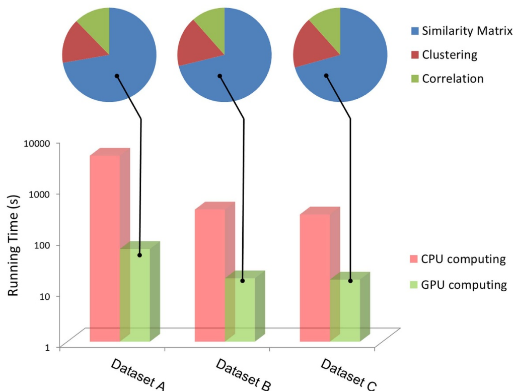
Figure 8 | Running time for the whole data-mining procedures. Bar chart illustrated the running time comparison between CPU (16 core) and GPU (Tesla M2075) computing. The Y-axis was in 10-based log scale. Pie charts showed the proportions of each processing step in the total running time.
