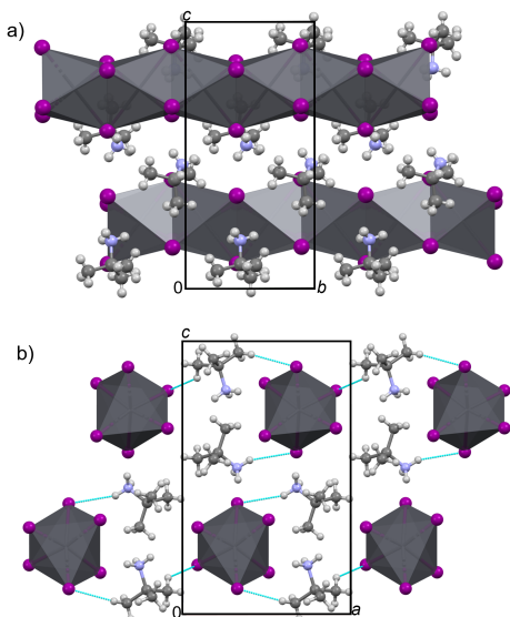
Figure 3. The 1D structure of ( t -BA)PbI 3 in a) bc plane and b) ac plane. Iodide is given in purple, lead in dark grey, carbon in light grey, nitrogen in pale blue while hydrogen atoms are shown in white. Hydrogen bonds are shown as dashed turquoise lines. Organic cations are disordered between several positions; only the major part is shown.
