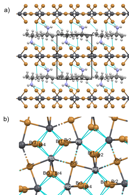
Figure 4. a) The 2D structure of ( t -BA) 2 Pb 2 Br 5 in ac plane and b) inorganic layer consisting of PbBr 8 bicapped trigonal prisms (caps at Br5 atoms). Bromide is given in dark orange, lead in dark grey, carbon in light grey, nitrogen in pale blue while hydrogen atoms are shown in white. Hydrogen bonds are shown as dashed turquoise lines. Organic cations are disordered between several positions; only the major part is shown.
