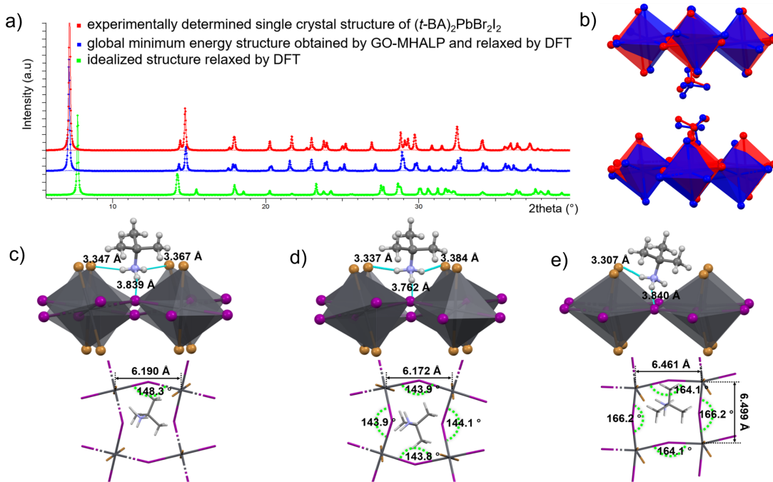
Figure 7. a) XRD patterns simulated from the experimental single-crystal structure and those predicted with and without GO-MHALP. b) Single-crystal structure (red) and global minimum energy structure predicted by GO-MHALP (blue) shown in an overlapping manner. Hydrogen atoms are omitted for clarity. Structural features of c) experimental structure and those predicted d) with GO-MHALP and e) without GO-MHALP. Bromide is given in dark orange, iodide in purple, lead in dark grey, carbon in light grey, nitrogen in pale blue while hydrogen atoms are shown in white. Hydrogen bonds are shown as dashed turquoise lines.
