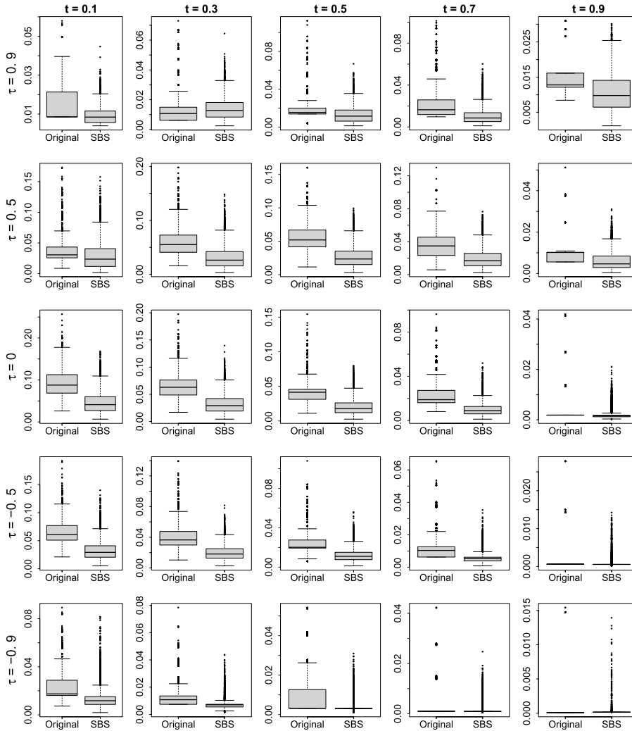
FIG 6. Hausdorff distance simulation results between the true and estimated level sets for a Clayton copula C_\theta with \theta such that \tau(C_\theta) \in \{-0.9, -0.5, 0, 0.5, 0.9\} , for levels t \in \{0.1, 0.3, 0.5, 0.7, 0.9\} . Original sample size n = 50 , augmented smooth bootstrap sample size m = 5000 . Each boxplot is based on M = 10\,000 independent reruns.
