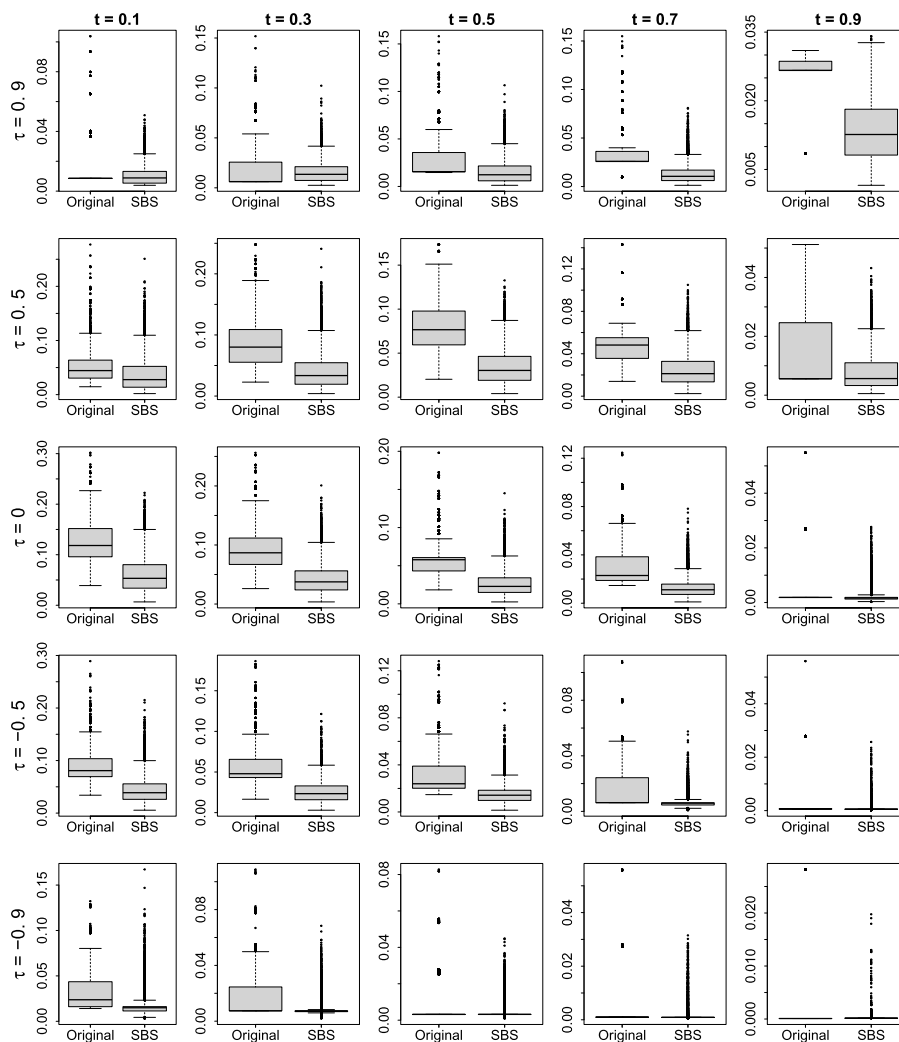
FIG 5. Hausdorff distance simulation results between the true and estimated level sets for a Clayton copula C_\theta with \theta such that \tau(C_\theta) \in \{-0.9, -0.5, 0, 0.5, 0.9\} , for levels t \in \{0.1, 0.3, 0.5, 0.7, 0.9\} . Original sample size n = 25 , augmented smooth bootstrap sample size m = 5000 . Each boxplot is based on M = 10000 independent reruns.
