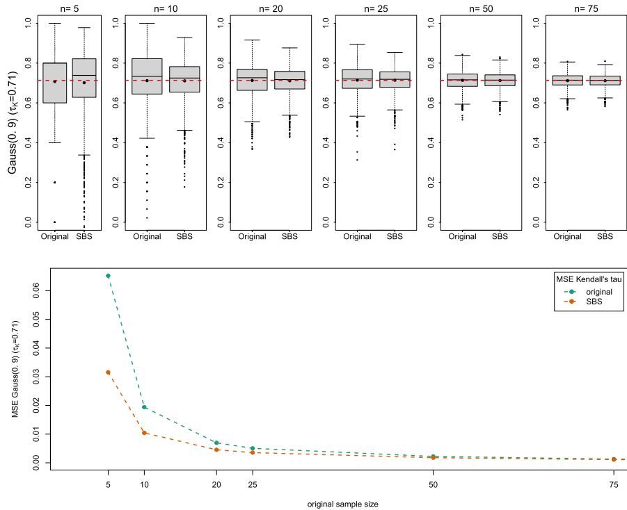
FIG 19. Top: Estimated Kendall's tau for the bivariate Gaussian copula with \rho = 0.9 . The results are based on an original sample size of n \in \{5, 10, 20, 25, 50, 75\} , while the augmented smooth bootstrap sample size is m = 10000 . Each boxplot is based on M = 2000 independent reruns. The red dashed line indicates the theoretical value of \tau_K while black dots indicate the means.
