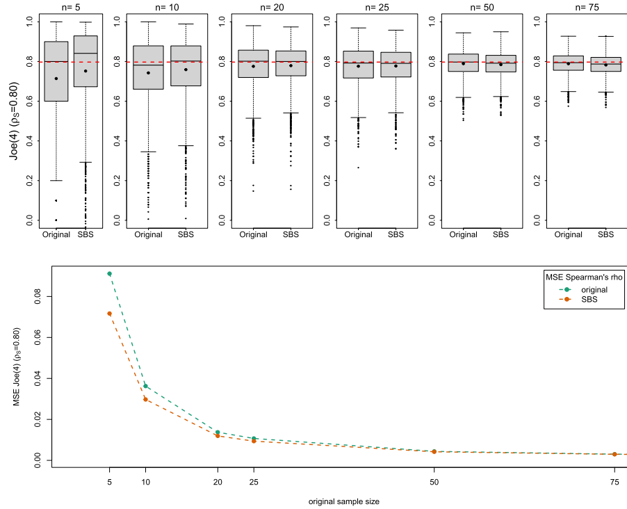
FIG 16. Top: Estimated Spearman’s rho for the bivariate Joe copula with parameter \theta = 4 . The results are based on an original sample size of n \in \{5, 10, 20, 25, 50, 75\} , while the augmented smooth bootstrap sample size is m = 10\,000 . Each boxplot is based on M = 2\,000 independent reruns. The red dashed line indicates the theoretical value of \rho_S while black dots indicate the means. Bottom: Mean squared error for estimation of Spearman’s rho. The results are based on an original sample size of n \in \{5, 10, 20, 25, 50, 75\} , while the augmented smooth bootstrap sample size is m = 10\,000 .
