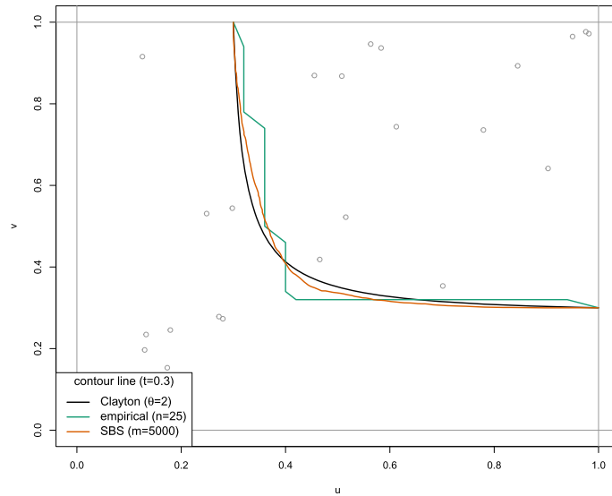
FIG 8. Theoretical (black) and estimated contour lines for a Clayton copula with parameter \theta = 2 at level t = 0.3 . Direct estimation (green) is based on n = 25 sample points. For the smooth bootstrap (orange) m = 5\,000 pseudo-observations are generated based on the initial sample.
