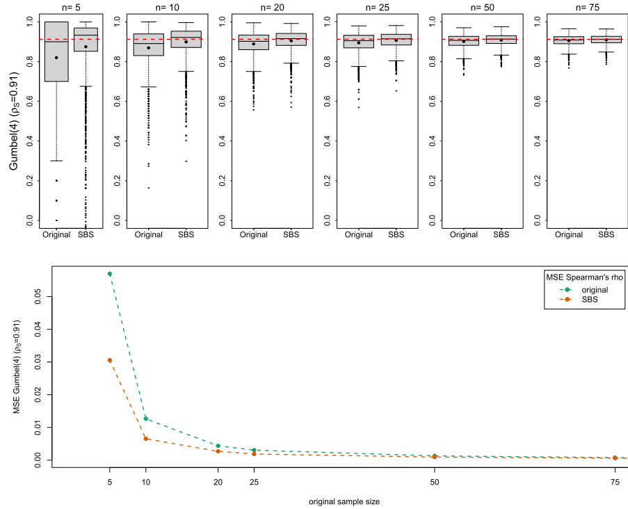
FIG 14. Top: Estimated Spearman's rho for the bivariate Gumbel copula with parameter \theta = 4 . The results are based on an original sample size of n \in \{5, 10, 20, 25, 50, 75\} , while the augmented smooth bootstrap sample size is m = 10\,000 . Each boxplot is based on M = 2\,000 independent reruns. The red dashed line indicates the theoretical value of \rho_S while black dots indicate the means.
