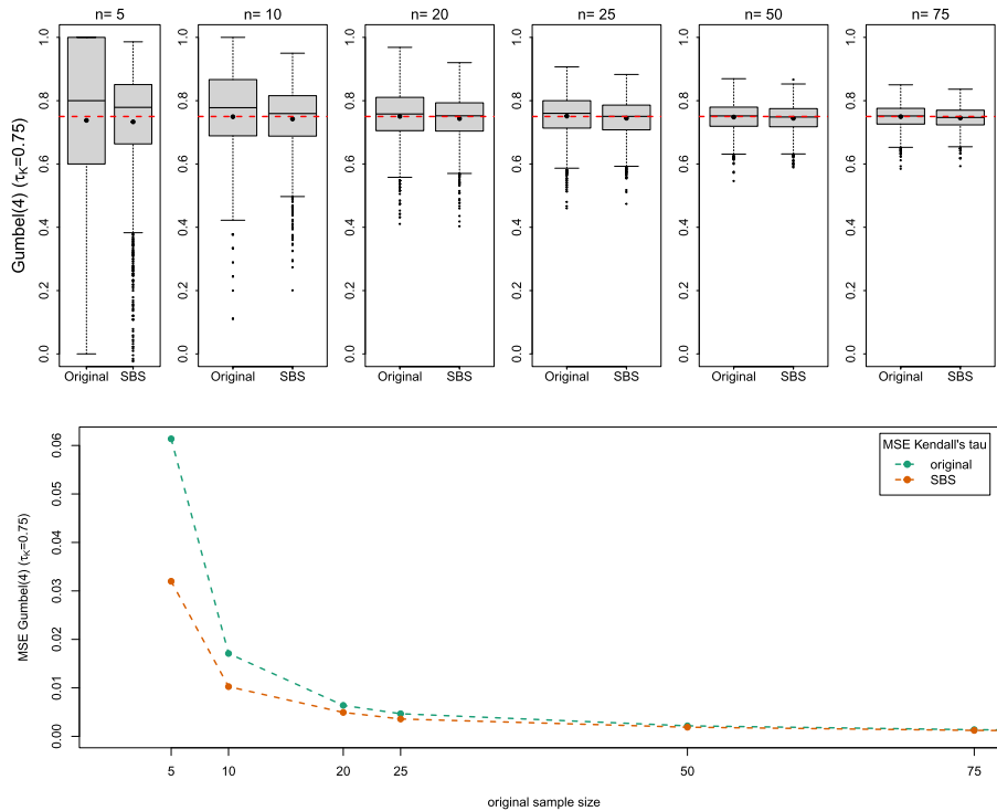
FIG 15. Top: Estimated Kendall's tau for the bivariate Gumbel copula with parameter \theta = 4 . The results are based on an original sample size of n \in \{5, 10, 20, 25, 50, 75\} , while the augmented smooth bootstrap sample size is m = 10000 . Each boxplot is based on M = 2000 independent reruns. The red dashed line indicates the theoretical value of \tau_K while black dots indicate the means. Bottom: Mean squared error for estimation of Kendall's tau. The results are based on an original sample size of n \in \{5, 10, 20, 25, 50, 75\} , while the augmented smooth bootstrap sample size is m = 10000 .
