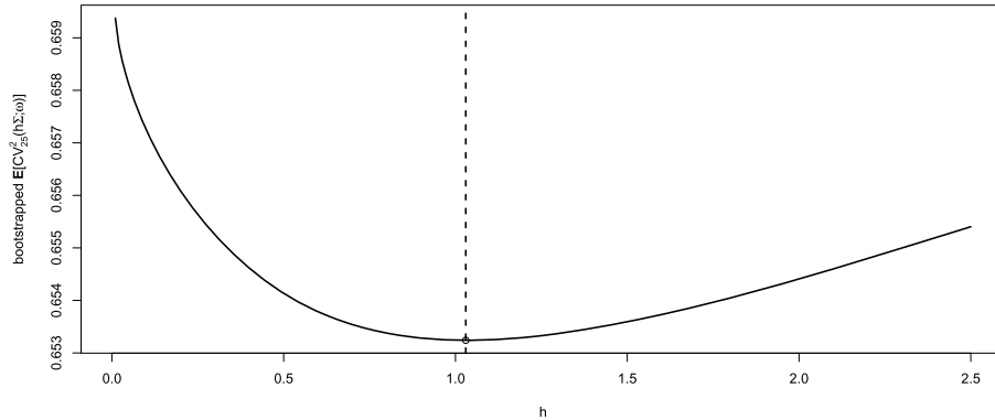
FIG 4. Bootstrapped version of \mathbb{E}[CV_{25}^2(h\Sigma; w)] based on the sample \mathbb{X}_1 over a grid h \in \{0.01, 0.02, \dots, 2.5\} . The approximation is based on 25 independent bootstrap samples drawn from \mathbb{X}_1 . The minimum is indicated by a circle and the dashed vertical line.
