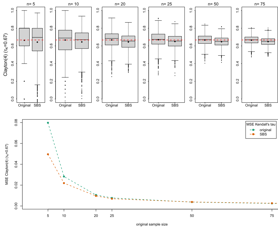
FIG 11. Top: Estimated Kendall's tau for the bivariate Clayton(4) copula. The results are based on an original sample size of n \in \{5, 10, 20, 25, 50, 75\} , while the augmented smooth bootstrap sample size is m = 10000 . Each boxplot is based on M = 2000 independent reruns. The red dashed line indicates the theoretical value of \tau_K while black dots indicate the means. Bottom: Mean squared error for estimation of Kendall's tau for the bivariate Clayton(4) copula. The results are based on an original sample size of n \in \{5, 10, 20, 25, 50, 75\} , while the augmented smooth bootstrap sample size is m = 10000 .
