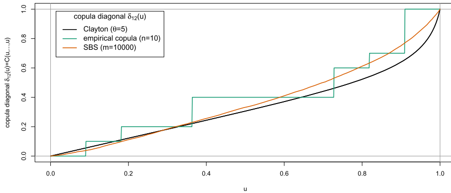
FIG 9. Theoretical (black) and estimated copula diagonal for a twelve dimensional Clayton copula with parameter \theta = 5 . Direct estimation (green) via the empirical copula is based on n = 10 sample points. For the smooth bootstrap (orange) m = 10\,000 pseudo-observations are generated based on the initial sample which are then used to estimate the diagonal via the empirical copula.
