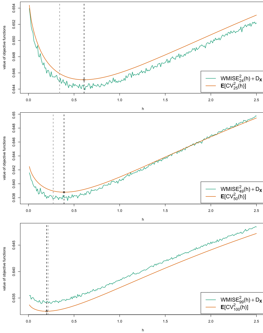
FIG 2. Numerical approximation of \mathbb{E}[\text{CV}_n^2(H; w)] (orange) and \text{WISE}_{n-1}^2(H; w) + D_{\mathbf{X}} (green) for n = 25 (top), n = 50 (middle) and n = 100 (bottom) with H = h\Sigma for h \in \{0.01, 0.02, \dots, 2.5\} . The minimum of \mathbb{E}[\text{CV}_n^2(H; w)] is indicated by a circle and the dashed vertical black line in all cases. The dashed vertical gray line indicates the choice of h following Silverman's rule of thumb.
