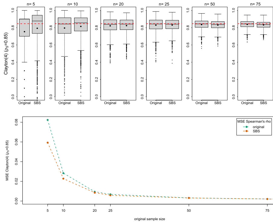
FIG 10. Top: Estimated Spearman's rho for the bivariate Clayton(4) copula. The results are based on an original sample size of n \in \{5, 10, 20, 25, 50, 75\} , while the augmented smooth bootstrap sample size is m = 10\,000 . Each boxplot is based on M = 2\,000 independent reruns. The red dashed line indicates the theoretical value of \rho_S while black dots indicate the means. Bottom: Mean squared error for estimation of Spearman's rho for the bivariate Clayton(4) copula. The results are based on an original sample size of n \in \{5, 10, 20, 25, 50, 75\} , while the augmented smooth bootstrap sample size is m = 10\,000 .
