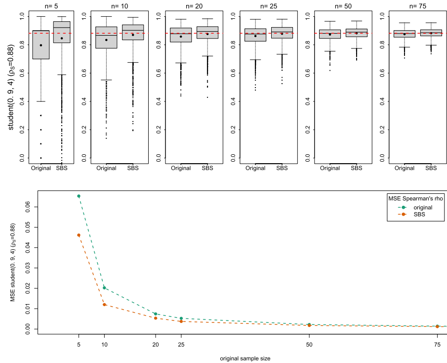
FIG 12. Top : Estimated Spearman's rho for the bivariate Student- t copula with \rho = 0.9 and \nu = 4 degrees of freedom. The results are based on an original sample size of n \in \{5, 10, 20, 25, 50, 75\} , while the augmented smooth bootstrap sample size is m = 10000 . Each boxplot is based on M = 2000 independent reruns. The red dashed line indicates the theoretical value of \rho_S while black dots indicate the means.
