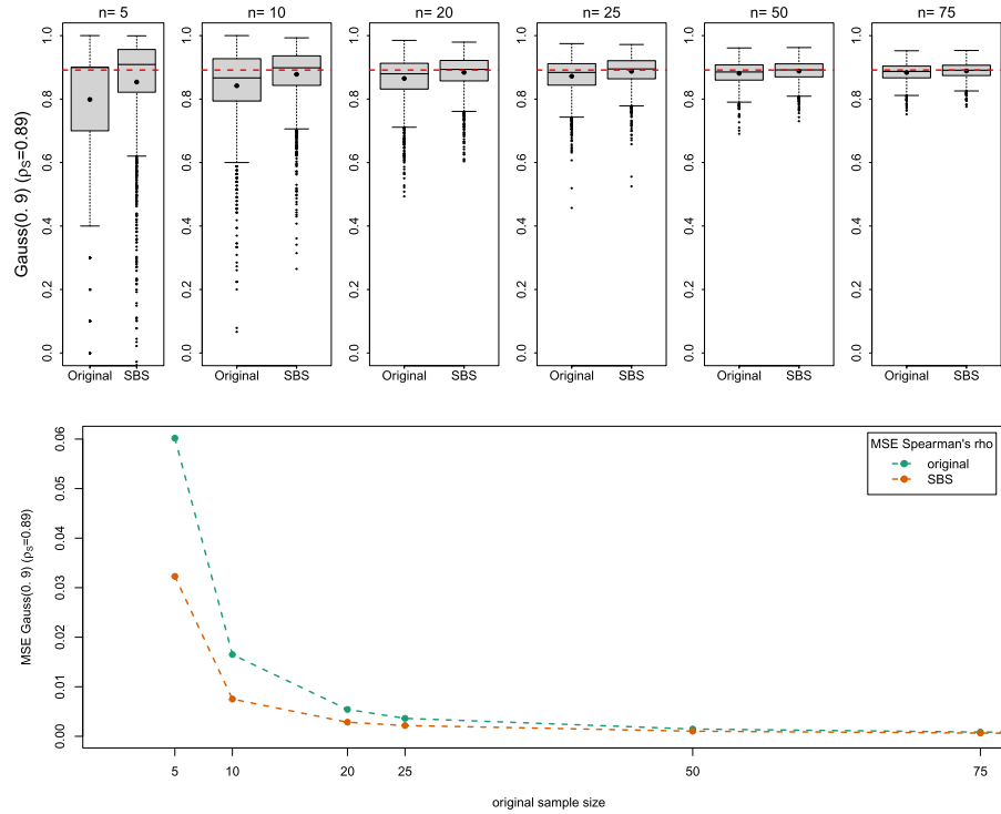
FIG 18. Top: Estimated Spearman's rho for the bivariate Gaussian copula with \rho = 0.9 . The results are based on an original sample size of n \in \{5, 10, 20, 25, 50, 75\} , while the augmented smooth bootstrap sample size is m = 10000 . Each boxplot is based on M = 2000 independent reruns. The red dashed line indicates the theoretical value of \rho_S while black dots indicate the means.
