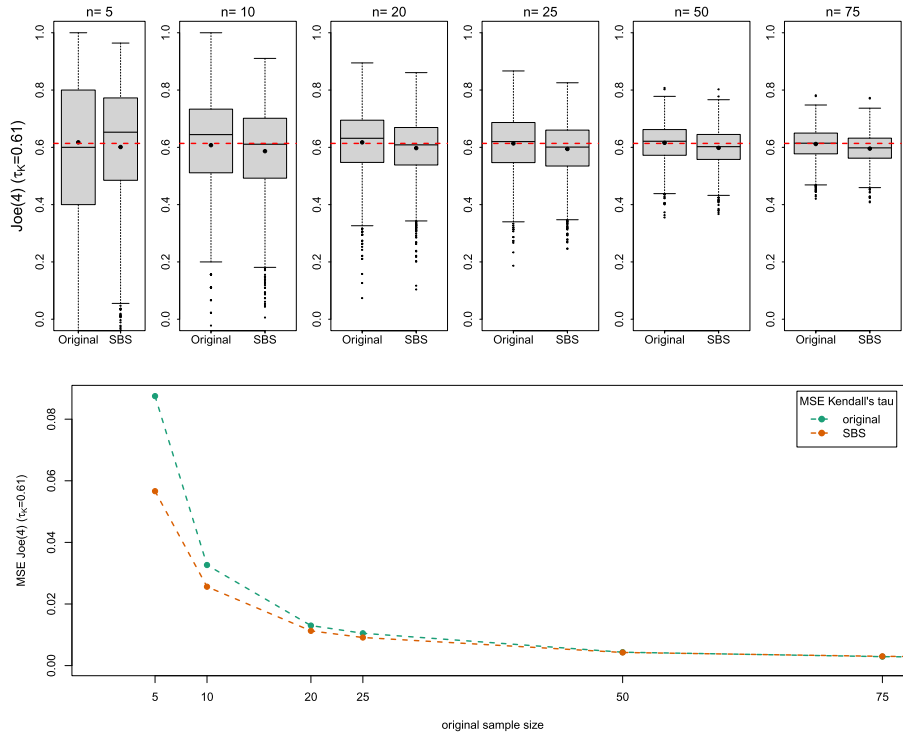
FIG 17. Top: Estimated Kendall’s tau for the bivariate Joe copula with parameter \theta = 4 . The results are based on an original sample size of n \in \{5, 10, 20, 25, 50, 75\} , while the augmented smooth bootstrap sample size is m = 10000 . Each boxplot is based on M = 2000 independent reruns. The red dashed line indicates the theoretical value of \tau_K while black dots indicate the means.
