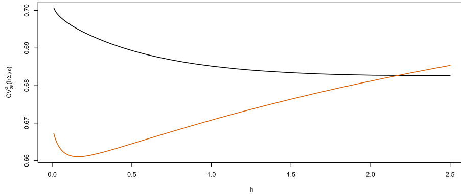
FIG 3. CV_{25}^2(h\Sigma; w) for two independent samples \mathbb{X}_1 = \{\mathbf{X}_i\}_{i=1}^{25} (black) and \mathbb{X}_2 = \{\mathbf{X}_i\}_{i=1}^{25} (orange) of \mathbf{X} over a grid h \in \{0.01, 0.02, \dots, 2.5\} .
