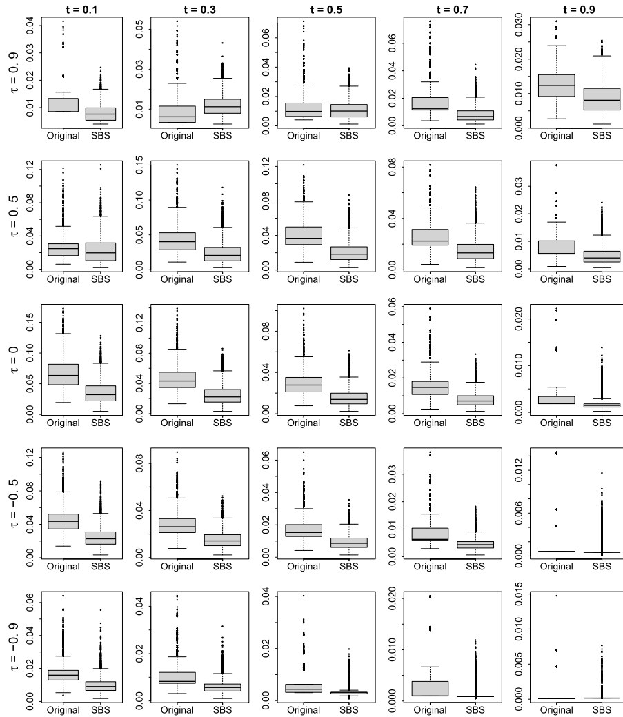
FIG 7. Hausdorff distance simulation results between the true and estimated level sets for a Clayton copula C_\theta with \theta such that \tau(C_\theta) \in \{-0.9, -0.5, 0, 0.5, 0.9\} , for levels t \in \{0.1, 0.3, 0.5, 0.7, 0.9\} . Original sample size n = 100 , augmented smooth bootstrap sample size m = 5000 . Each boxplot is based on M = 10000 independent reruns.
