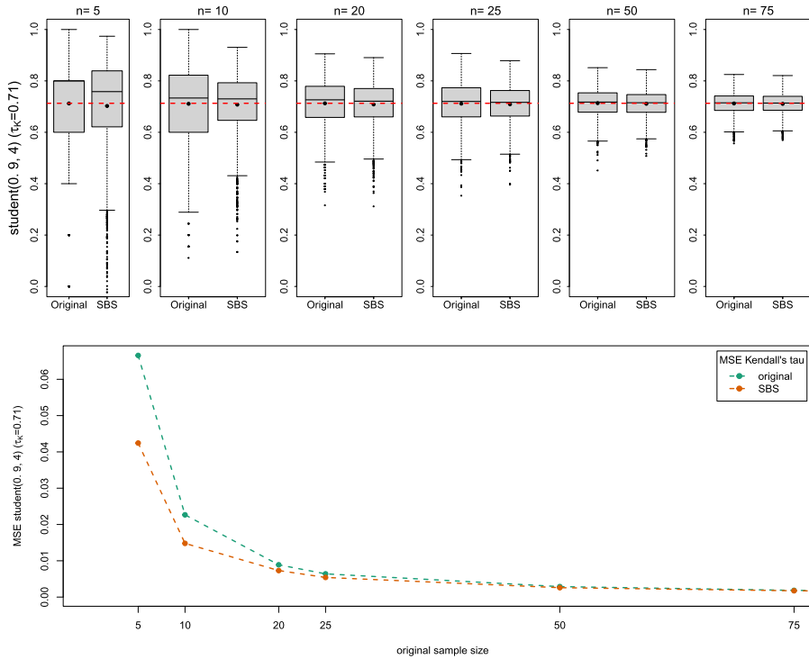
FIG 13. Top: Estimated Kendall's tau for the bivariate Student-t copula with \rho = 0.9 and \nu = 4 degrees of freedom. The results are based on an original sample size of n \in \{5, 10, 20, 25, 50, 75\} , while the augmented smooth bootstrap sample size is m = 10000 . Each boxplot is based on M = 2000 independent reruns. The red dashed line indicates the theoretical value of \tau_K while black dots indicate the means. Bottom: Mean squared error for estimation of Kendall's tau. The results are based on an original sample size of n \in \{5, 10, 20, 25, 50, 75\} , while the augmented smooth bootstrap sample size is m = 10000 .
