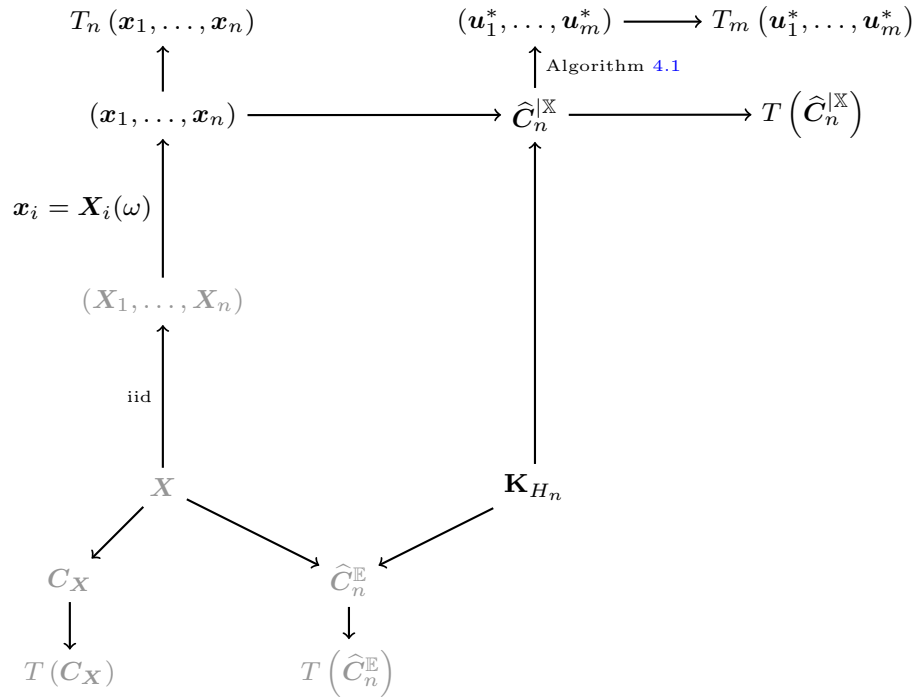
FIG 1. Schematic relationships between the objects under consideration. Objects in gray are at the (inaccessible) population level, while objects in black are tangible to the statistician. C_X is the theoretical copula, \hat{C}_n^E the theoretical copula constructed by convolving the underlying joint distribution F_X with the kernel K_{H_n} , and \hat{C}_n^X the smoothed copula. T and T_n denote the population version and estimated version of the considered functional, respectively.
