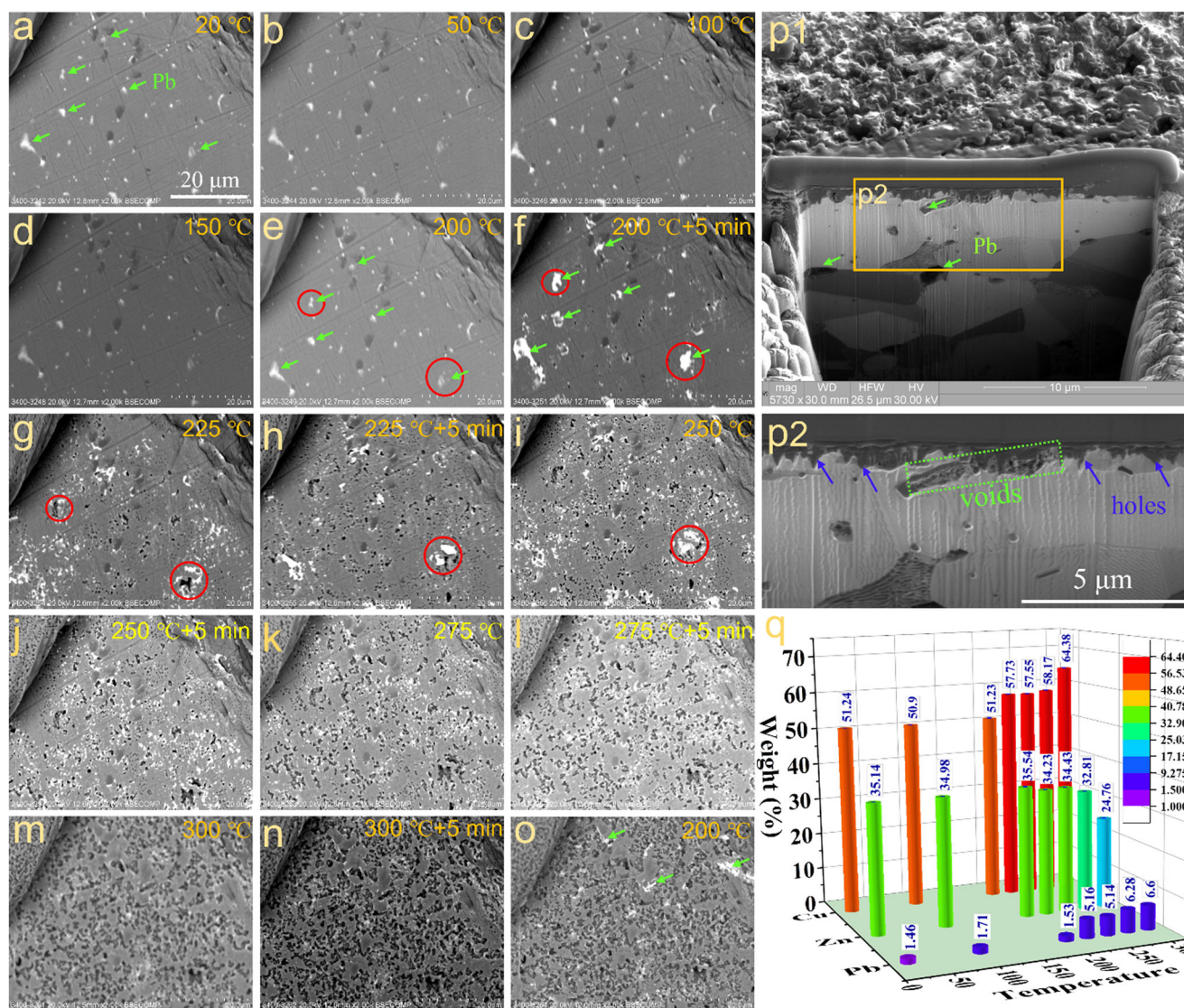
Fig. 7 Pb surfacing during in situ heating. The imaging was conducted by heating the brass samples at 50 °C increments from room temperature to 200 °C, followed by 25 °C increments between 200 and 300 °C, and holding each temperature for 5 min inside an SEM in a vacuum state, followed by a decrease in temperature to 200 °C for 5 min (a–o). The heated samples were then cut open with FIB (Fig. 7p1). Figure 7q shows the content of Pb on the heating surface detected by SEM-EDS.
