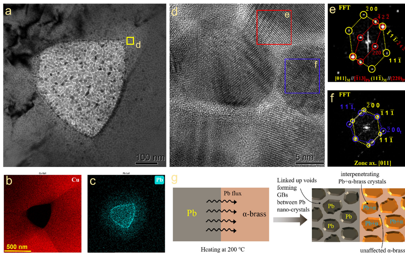
Fig. 4 TEM analysis of a Pb particle at triple point of brass grains in a sample heated to 200 °C for 5 min. a TEM bright-field image of the particle and its surrounding. b, c Element maps. d HRTEM image of the brass matrix in the frame marked in (a). e, f FFT of the HRTEM image in the corresponding frames in (d). g Schematic showing the formation of the observed microstructure.
