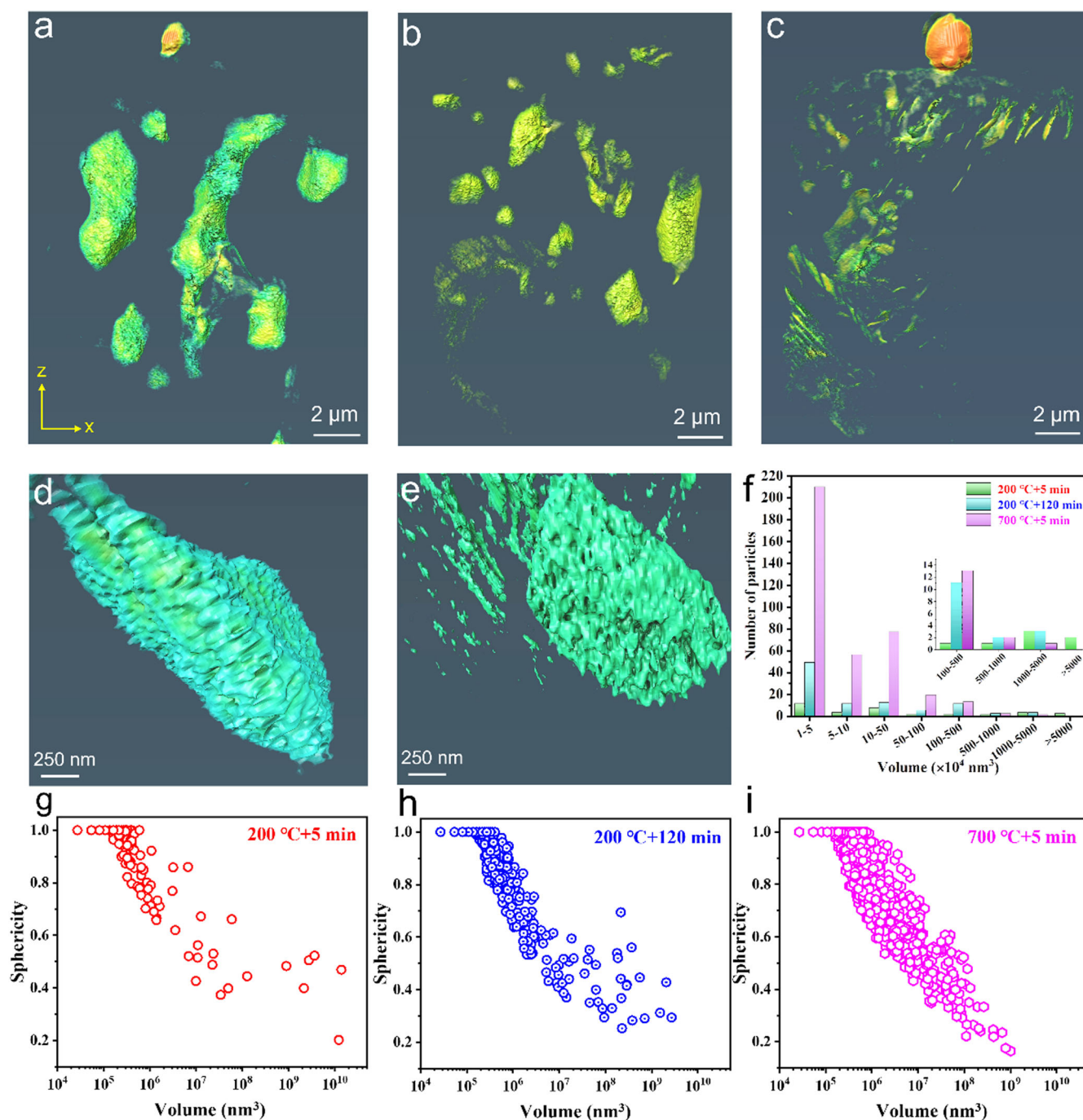
Fig. 3 Results of synchrotron radiation X-ray imaging. a Sample heated at 200 °C for 5 min (hide brass to see the 3D distribution of Pb). b Sample heated at 200 °C for 120 min. c Sample heated at 700 °C for 5 min. d High magnification of the picture for the sample heated at 200 °C for 5 min. e High magnification of the picture for the sample heated at 700 °C for 5 min. f Size distribution of lead particles. g–i Shape distribution of lead particles (the extent to which different sizes of lead particles are close to spherical shape).
