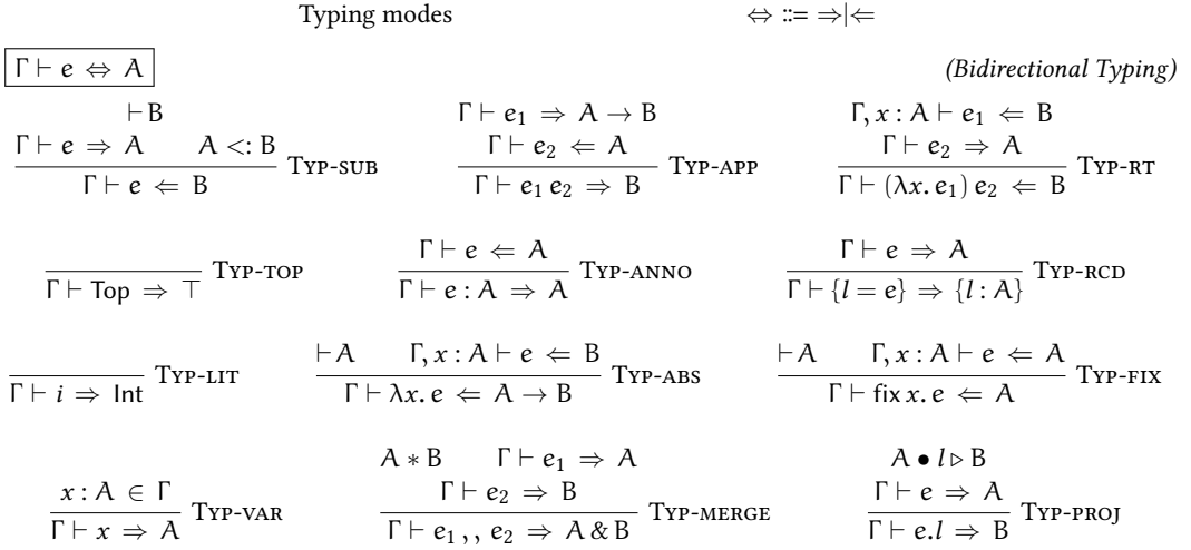
Fig. 3. The type system of the \lambda M calculus.
