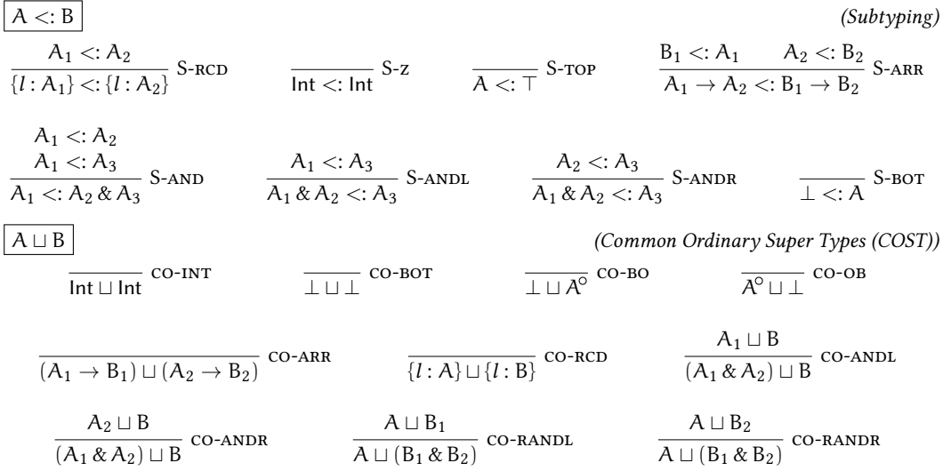
Fig. 4. Subtyping and the COST.
