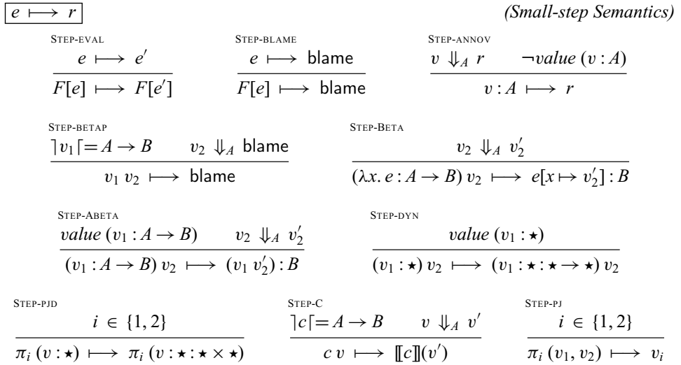
Fig. 5. Semantics of \lambda B^g .
