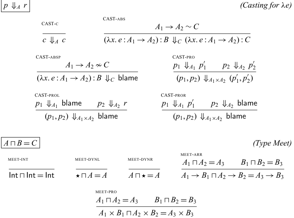
Fig. 16. Casting for the \lambda e calculus.
