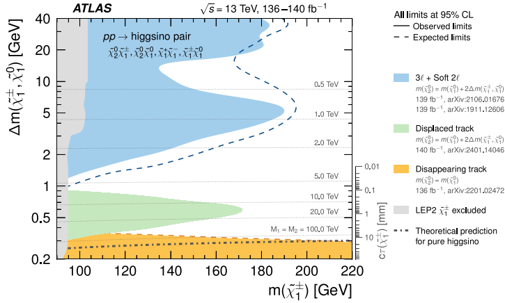
Fig. 15. Exclusion limits for higgsino pair production \tilde{\chi}_1^+ \tilde{\chi}_1^- , \tilde{\chi}_1^\pm \tilde{\chi}_1^0 , \tilde{\chi}_1^\pm \tilde{\chi}_2^0 , and \tilde{\chi}_1^0 \tilde{\chi}_2^0 with off-shell SM-boson-mediated decays to the lightest neutralino, \tilde{\chi}_1^0 , as a function of the \tilde{\chi}_1^\pm and \tilde{\chi}_1^0 masses. The production cross-section is for pure higgsinos. Where more than one reference is given for each line, the total exclusion limit from multiple analyses is shown. The LEP2 \tilde{\chi}_1^\pm exclusion is taken from Ref. [71].
