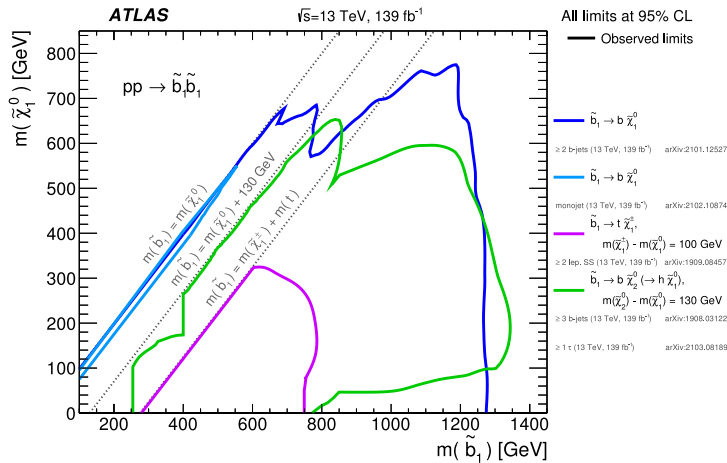
Fig. 9. Exclusion limits in the m(\tilde{b}_1) – m(\tilde{\chi}_1^0) plane for direct sbottom production. The lightest neutralino ( \tilde{\chi}_1^0 ) is assumed to be the LSP. Several different decay scenarios are shown, along with different parameterisations of the intermediate particles in the models. Where more than one reference is given for each line, the total exclusion limit from multiple analyses is shown.
