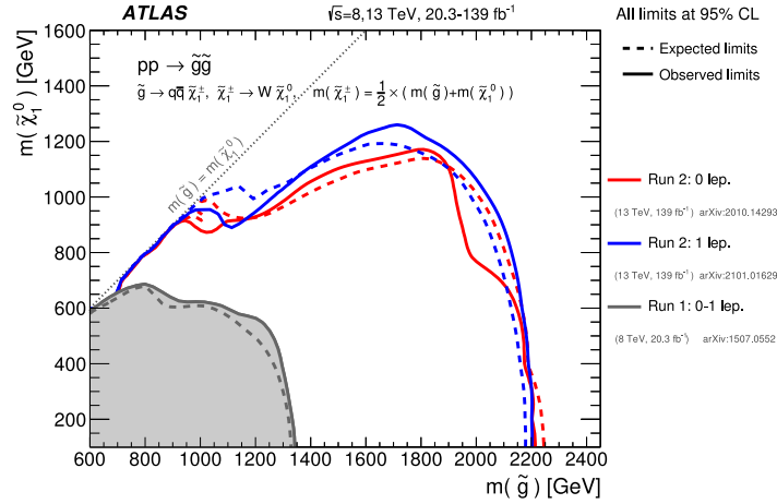
Fig. 6. Exclusion limits from 13 TeV data in the m(\tilde{g}) – m(\tilde{\chi}_1^0) plane for the simplified model where a pair of gluinos are produced, and each decays promptly via an on-shell chargino into a pair of quarks, a W boson, and the lightest neutralino. The chargino mass is assumed to be midway between the gluino and neutralino masses. Theoretical signal cross-section uncertainties are not included in the limits shown.
