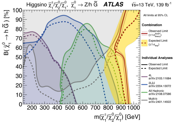
Fig. 16. Exclusion limits in a General Gauge Mediation model from 13 TeV data. The model assumes a pure-higgsino NLSP that promptly decays into either a Z boson and gravitino or a Higgs boson and gravitino. The limits are displayed as a function of the mass of the nearly mass-degenerate higgsino multiplet and the branching fraction of the lightest higgsino into a Higgs boson and gravitino.
