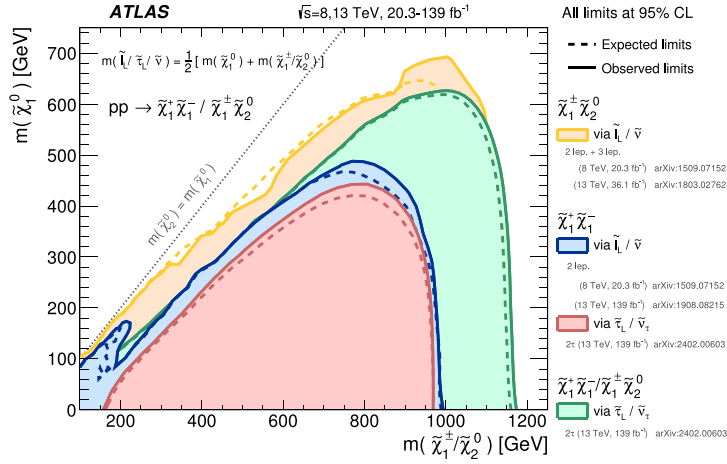
Fig. 12. The exclusion limits on \tilde{\chi}_1^\pm \tilde{\chi}_1^\mp and \tilde{\chi}_1^\pm \tilde{\chi}_2^0 production with \tilde{l} -mediated decays, as a function of the \tilde{\chi}_1^\pm , \tilde{\chi}_2^0 and \tilde{\chi}_1^0 masses. The production cross-section is for pure-wino \tilde{\chi}_1^\pm \tilde{\chi}_1^\mp and \tilde{\chi}_1^\pm \tilde{\chi}_2^0 . Where more than one reference is given for each line, the total exclusion limit from multiple analyses is shown.
