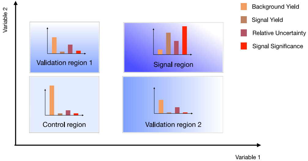
Fig. 4. Illustrative set-up for an analysis using two variables as the final discriminant. The definition of mutually exclusive signal, control and validation regions is sketched, and indicative values for the signal and background yields, relative uncertainty and signal significance in each region are shown (on an arbitrary scale).
