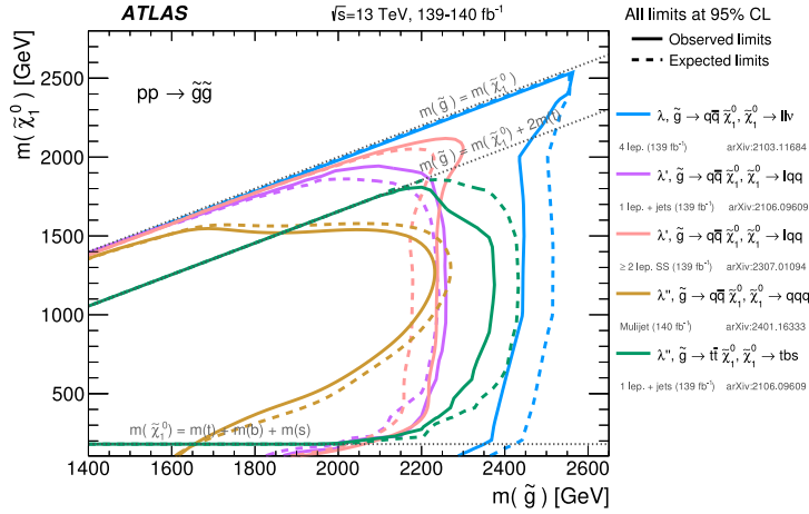
Fig. 17. Exclusion limits at 95% CL based on 13 TeV data in the (\tilde{g}, \tilde{\chi}_1^0) mass plane for different simplified models featuring the decay of the gluino to the lightest supersymmetric particle ( \tilde{\chi}_1^0 ) which in turn decays via R-parity-violating couplings to SM particles. For each line, the decay mode is reported in the legend and it is assumed to proceed with 100% branching fraction. Some limits depend on additional assumptions, as described in the references cited in the plot.
