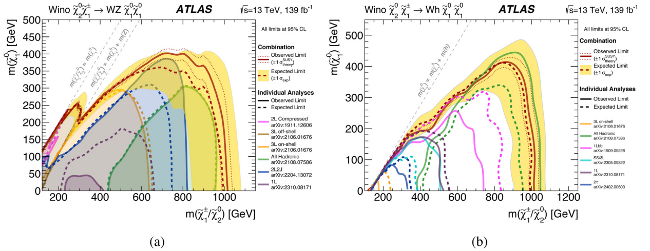
Fig. 14. The exclusion limits on \tilde{\chi}_1^\pm \tilde{\chi}_2^0 production with \tilde{\chi}_1^\pm \rightarrow \tilde{\chi}_1^0 W^\pm and (a) \tilde{\chi}_2^0 \rightarrow \tilde{\chi}_1^0 Z or (b) \tilde{\chi}_2^0 \rightarrow \tilde{\chi}_1^0 h , as a function of the \tilde{\chi}_1^\pm , \tilde{\chi}_2^0 and \tilde{\chi}_1^0 masses. The production cross-section is for pure-wino \tilde{\chi}_1^\pm and \tilde{\chi}_2^0 . The labels with L and J denote the number of leptons and jets in the search, respectively.
