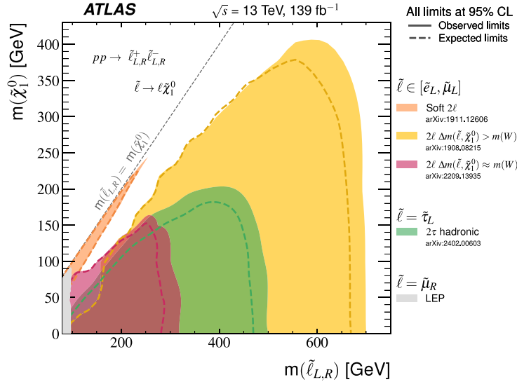
Fig. 11. Exclusion limits in the m(\tilde{\ell}) – m(\tilde{\chi}_1^0) plane for different analyses probing the direct production of sleptons with decays into a lepton and neutralino. The type of sleptons (flavour and coupling) included in each search is specified in the legend.
