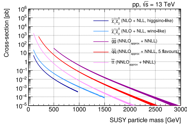
Fig. 2. Direct pair-production cross-sections for a few processes mediated by the strong or electroweak processes. The width of the line represents the theoretical uncertainty. The values of the cross-sections and uncertainties are those agreed upon by the LHC SUSY Cross Section Working Group [20].
