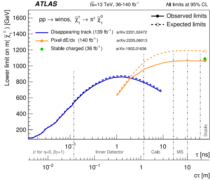
Fig. 18. Constraints on the \tilde{\chi}_1^\pm mass as a function of its lifetime for an AMSB model with \tan\beta = 5 and \mu > 0 . The wino-like \tilde{\chi}_1^\pm is pair-produced and decays into a wino-like \tilde{\chi}_1^0 and a very soft charged pion. The solid lines indicate the observed limits, while the dashed lines indicate the expected limits. The area below the curves is excluded. “Calo” and “MS” refer to the ATLAS calorimeter and muon spectrometer systems, respectively. The analyses also have sensitivity at lifetimes other than those shown, but only the limits at tested lifetimes are shown. The three markers at large lifetime represent results for which the particle is assumed to be stable. In this context, stable means escaping the detector. The exclusion contours from the pixel dE/dx search are each extrapolated to the stable regime with a straight line.
