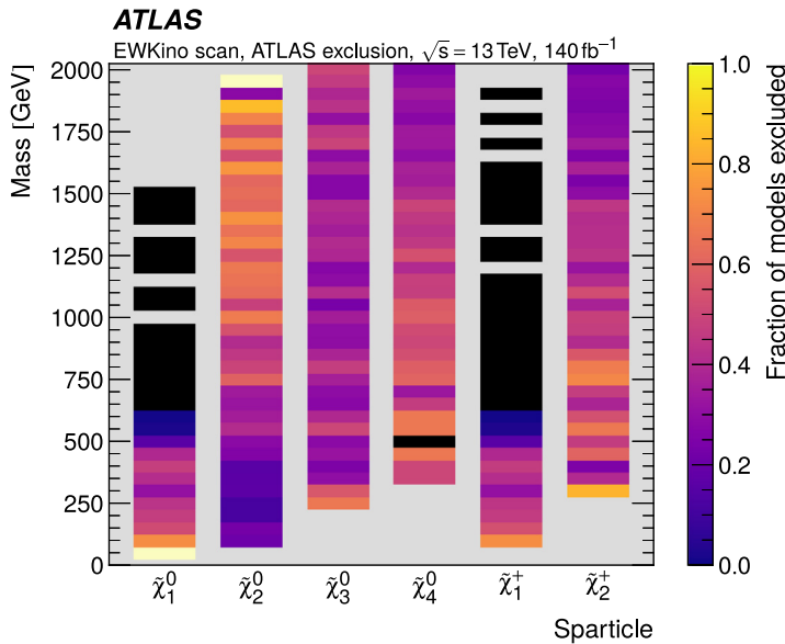
Fig. 20. Fraction of models passing external constraints but excluded by ATLAS, depending on the mass of the electroweakinos for the EWKino samples. Bins in grey indicate that no model passes external constraints, while for bins in cream (black) all models are (not) excluded.
