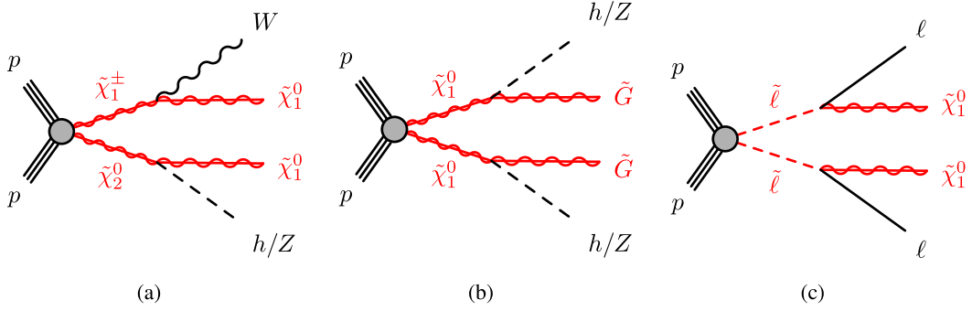
Fig. 3. Simplified models of (a) \tilde{\chi}_1^\pm \tilde{\chi}_2^0 production followed by \tilde{\chi}_1^\pm \rightarrow W^\pm \tilde{\chi}_1^0 , \tilde{\chi}_2^0 \rightarrow h/Z \tilde{\chi}_1^0 ; (b) \tilde{\chi}_1^0 \tilde{\chi}_1^0 production followed by \tilde{\chi}_1^0 \rightarrow h/Z \tilde{\chi}_1^0 ; (c) direct slepton pair production followed by \tilde{\ell} \rightarrow \ell \tilde{\chi}_1^0 . No distinction between particle and antiparticle is made in these diagrams.
