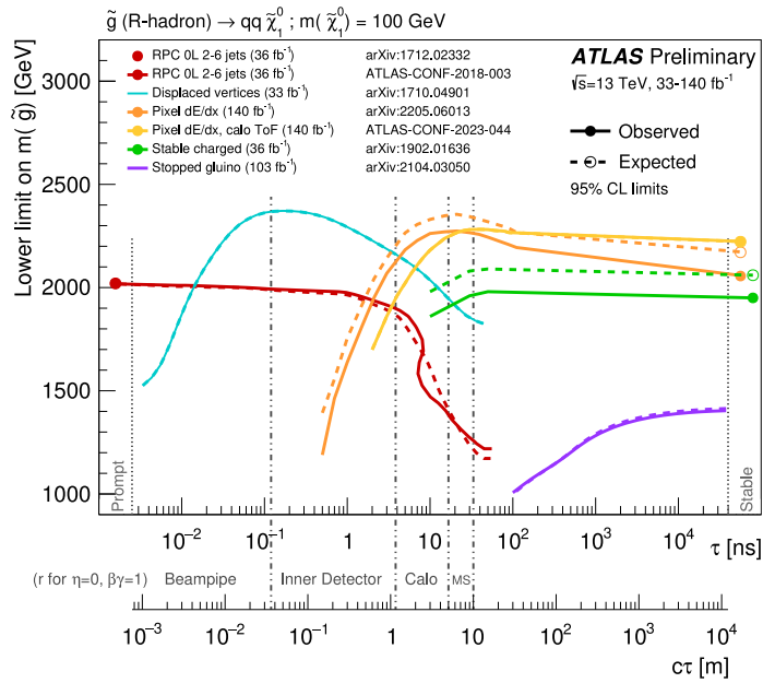
Fig. 19. Constraints on the gluino mass as a function of its lifetime for a split-supersymmetry model with the gluino R-hadron decaying into a gluon or light quarks and a neutralino with a mass of 100 GeV. The solid lines indicate the observed limits, while the dashed lines indicate the expected limits. The regions below the curves are excluded. “Calo” and “MS” refer to the ATLAS calorimeter and muon spectrometer systems, respectively, while “ToF” refers to the use of time of flight measurements. The expected and observed lines coincide for the Pixel dE/dx, calo ToF search. The markers at large lifetime represent results for which the particle is assumed to be stable. In this context, stable means escaping the detector.
