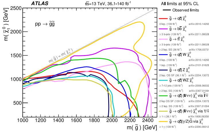
Fig. 5. Exclusion limits from 13 TeV data in the m(\tilde{g}) - m(\tilde{\chi}_1^0) plane for different simplified models featuring the decay of the gluino to the lightest supersymmetric particle (lightest neutralino or gravitino) either directly or through a cascade chain featuring other SUSY particles with intermediate masses. For each line, the gluino decay mode is reported in the legend and it is assumed to proceed with 100% branching fraction. Some limits depend on additional assumptions about the masses of intermediate states, as described in the references cited in the plot. Where more than one reference is given for each line, the total exclusion limit from multiple analyses is shown.
