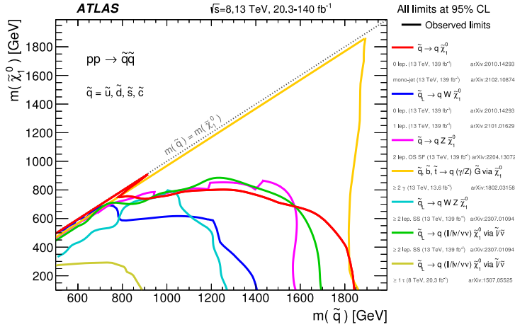
Fig. 8. Exclusion limits from 8 TeV and 13 TeV data in the m(\tilde{q}) – m(\tilde{\chi}_1^0) plane for different simplified models featuring the decay of squarks to the lightest supersymmetric particle (lightest neutralino or gravitino) either directly or through a cascade chain featuring other SUSY particles with intermediate masses. For each line, the squark decay mode is reported in the legend and it is assumed to proceed with 100% branching fraction. The limits on \tilde{q}_L \rightarrow q W \tilde{\chi}_1^0 assume the chargino mass to be midway between the squark and neutralino masses. The other \tilde{q}_L interpretations assume the first intermediate particle to be midway between the squark and neutralino masses, and the second intermediate particle to be midway between the first intermediate particle and neutralino masses. The additional assumptions about the masses of the intermediate states are described in the references cited in the plot. Where more than one reference is given for each line, the total exclusion limit from multiple analyses is shown.
