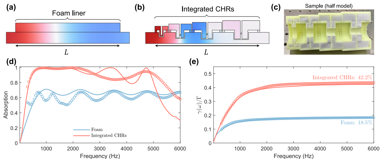
Fig. 5 | The characterization of a foam liner and the integrated CHRs. a, b The pressure fields of foam liner and integrated CHRs at 1000 Hz (simulated). The total thickness is the same, i.e., L = 14.1 cm. c The cross section of fabricated integrated CHRs (half model for the illustration). d Absorption performance comparison
