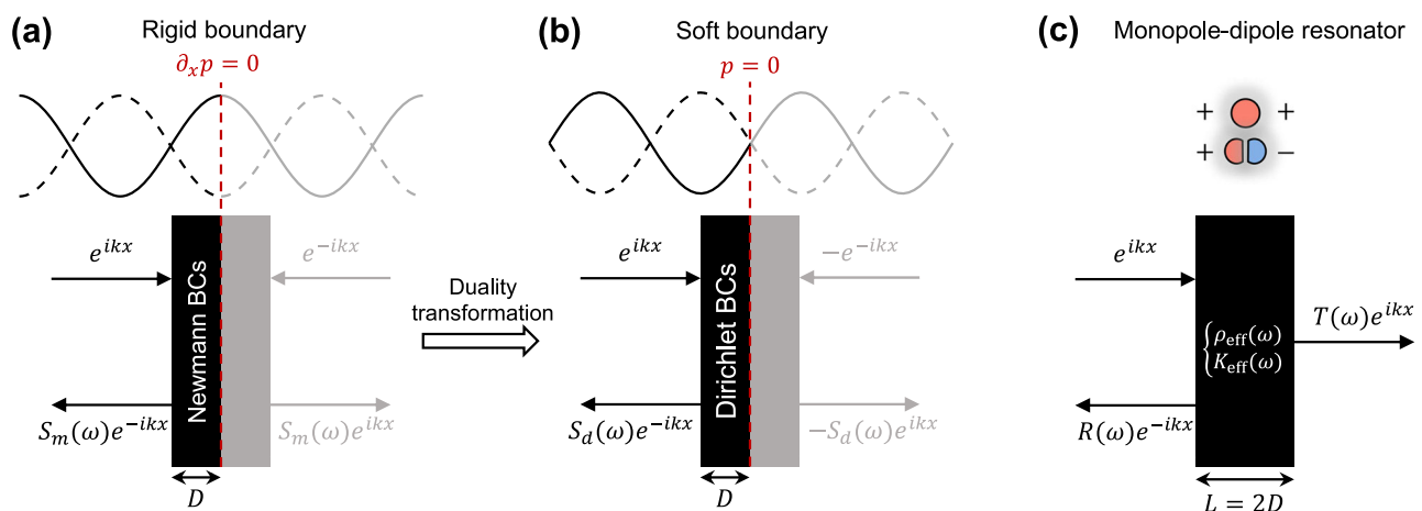
Fig. 1 | Wave scattering setups. a The monopole scattering with symmetrical pressure fields. b The dipole scattering with anti-symmetrical pressure fields. The sound fields in either half of the spaces in a , b can be applied to the causality
