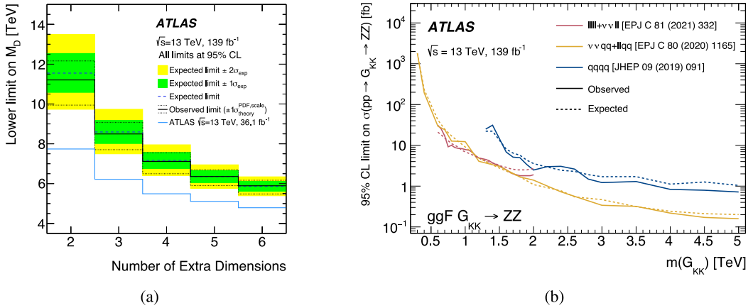
Fig. 49. Observed exclusion limit on (a) the fundamental scale M_D versus the number of extra dimensions in the ADD model, obtained by the jet+ E_T^{\text{miss}} analysis [242], and on (b) the cross section times branching ratio versus the mass of the graviton in a bulk RS model, obtained in the ZZ resonance searches [321].
