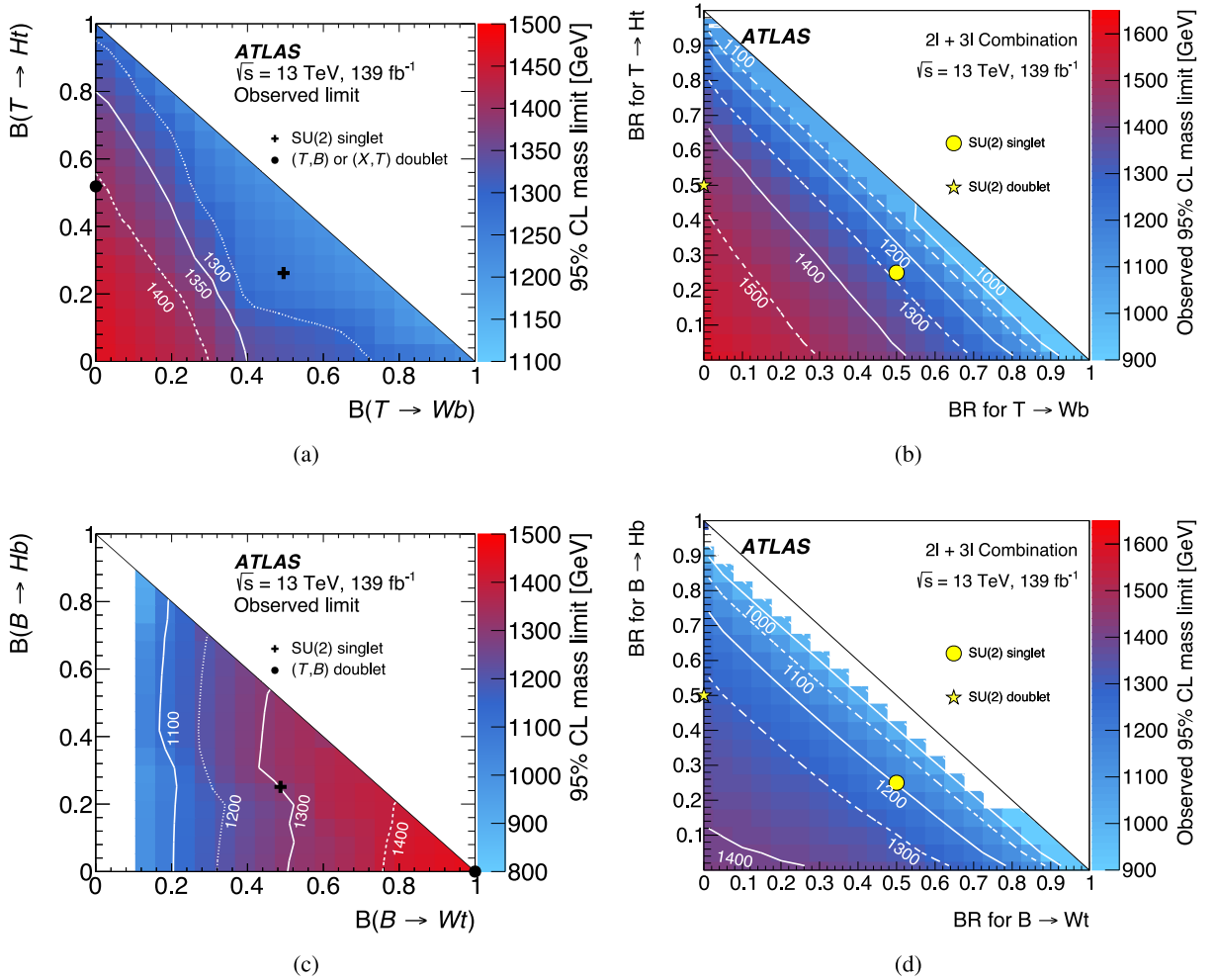
Fig. 13. Observed lower limits on the T and B masses in the BR plane for pair production of (a, b) TT and (c, d) BB . Results from (a,c) the search for VLQs in events with large E_T^{\text{miss}} [121] and (b,d) the search for pair-produced VLQs in multilepton final states [120] are included. The doublet hypothesis considered in (b,d) is (T, B) .
