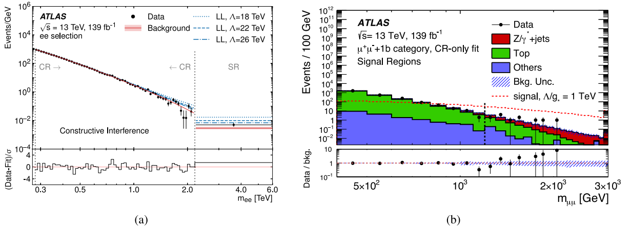
Fig. 33. Distribution of m_{\ell\ell} in the CR (where the data is fitted) and the SR (where the background estimate is an extrapolation from the fit) of the qq\ell\ell CI search [178], shown for (a) the ee channel with constructive interference, and (b) the bs\ell\ell search [180] in the \mu\mu channel with one b -tagged jet, where the region to the right of the dashed vertical line needs some fit-based extrapolation for the top background.
