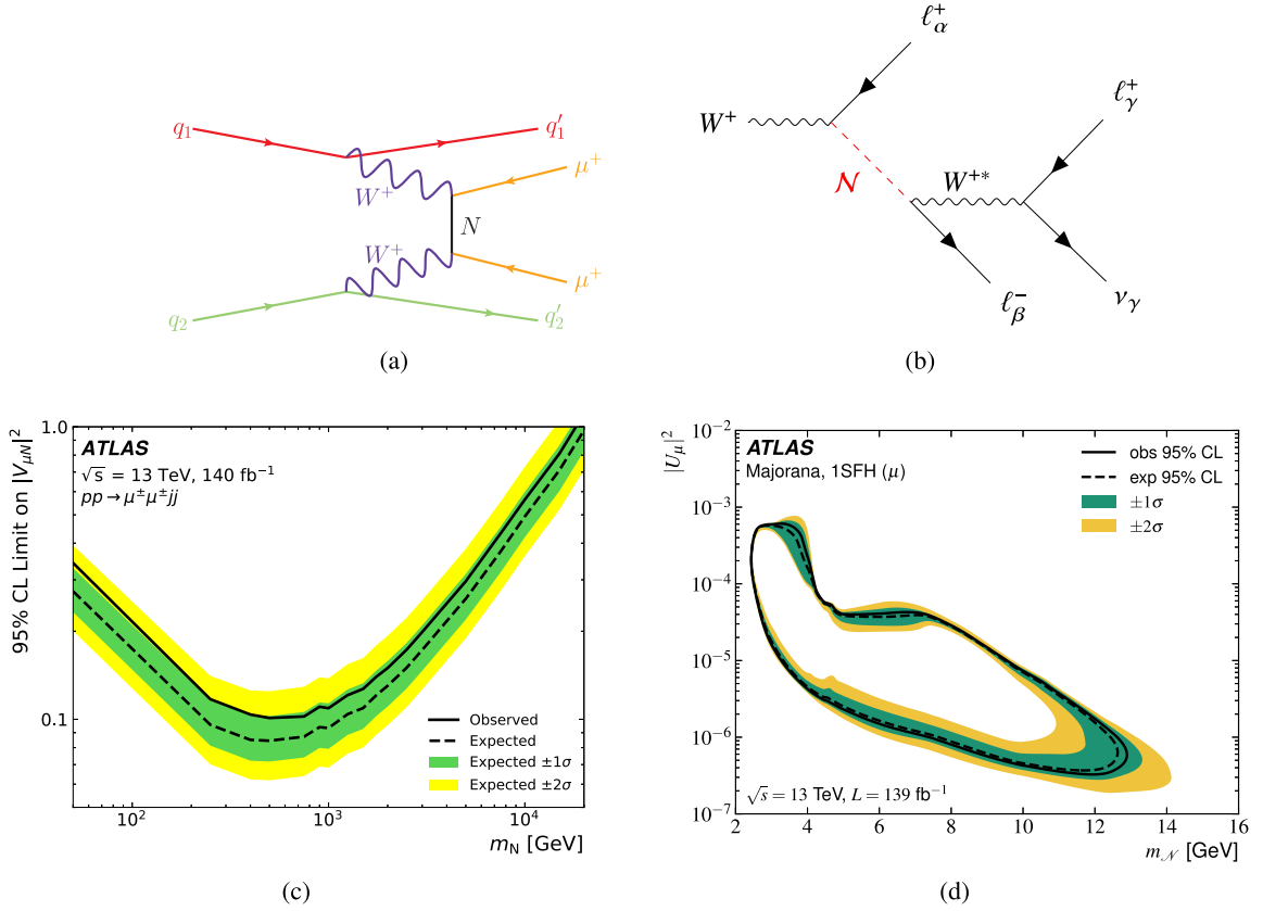
Fig. 4. Examples (a, b) of the production and decay of the heavy neutrinos and (c, d) limits set on the heavy Majorana neutrino mixing element |V_{\mu N}|^2 (also shown here as |U_{\mu}|^2 ) as a function of m_N in a Type-I seesaw mechanism by (a, c) the same-sign WW scattering search [88] and (b, d) the displaced dilepton vertex search [89].
