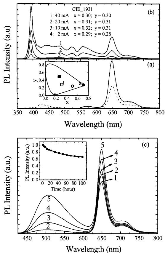
FIG. 3. (a) Emission spectra of the red LC-LED (solid line) doped with Alq 3 and without Alq 3 (dashed line). Inset: CIE_1931 chromaticity diagram, with coordinates corresponding to emission of the n -UV GaN LED (*), Alq 3 thin film (■), PtF 20 TPP thin film (●), red LC-LED doped with Alq 3 (×), red LC-LED without Alq 3 (○), the white LC-LED (□), and ideal pure white emission (+). (b) Emission spectra and CIE_1931 chromaticity coordinates of the white LC-LEDs under different applied currents. (c) PL spectra of PtF 20 TPP (1.0% in PC) as thin-film doped with Alq 3 (excited at 394 nm); (1) 1:0, (2) 1:2, (3) 1:5, (4) 1:10, (5) 1:20 (PtF 20 TPP:Alq 3 , by weight). Inset: photooxidative measurement of PtF 20 TPP film under irradiation of 1 mW/cm 2 at 394 nm in air at ambient temperature (signal detected at 650 nm).
