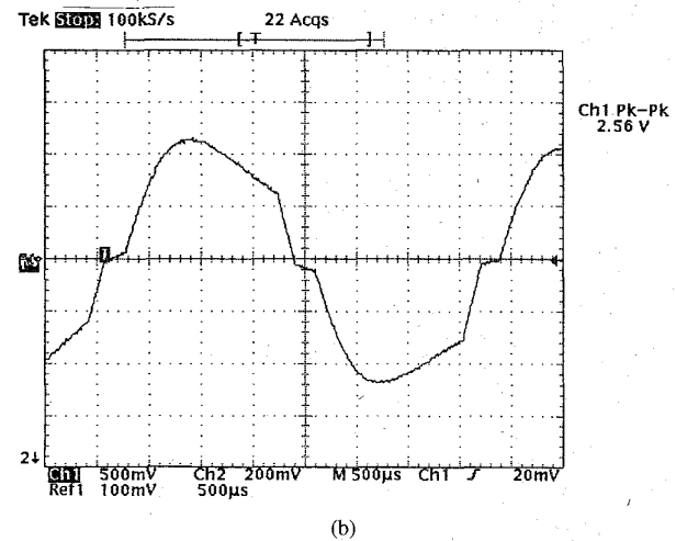
Fig. 7. Measured current waveforms. (a) Constant-torque operation at 500 rpm (20A/div, 1 ms/div). (b) Constant-power operation at 1500 rpm (10A/div, 500 \mu s/div).
