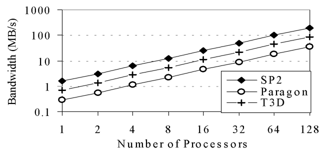
Fig. 7. Communication bandwidth of the El-Stag program.
