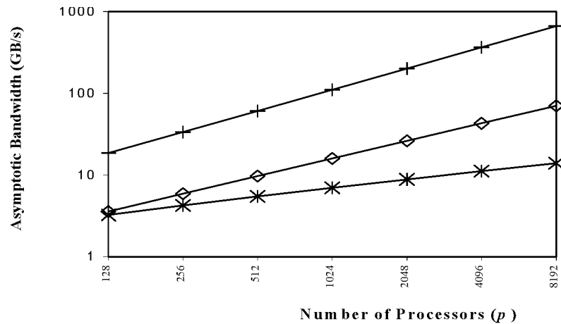
Fig. 12. Asymptotic bandwidth for total exchange on the ASCII machines.
