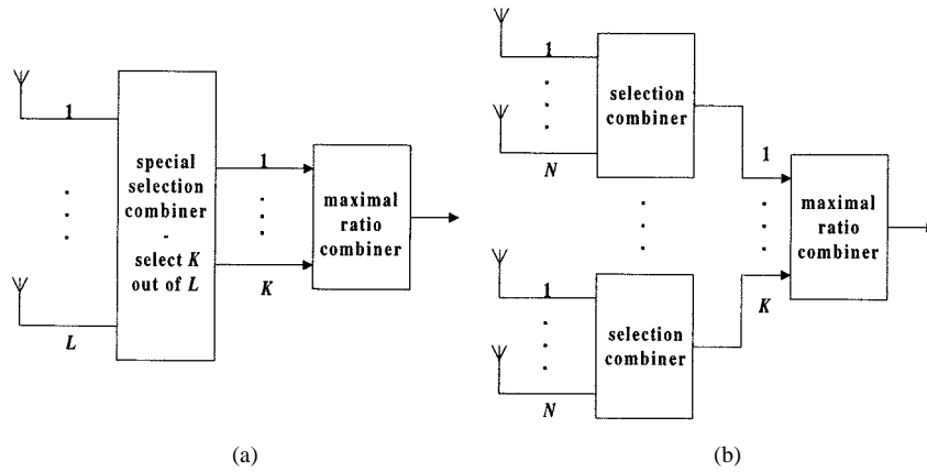
Fig. 1. Block diagrams for: (a) a generalized selection combining receiver and (b) a cascade combining receiver.
