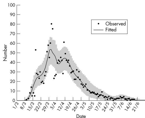
Figure 2 Observed and fitted number of SARS cases in Hong Kong Special Administrative Region.
