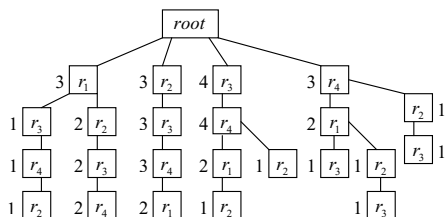
(a) Substring tree example
