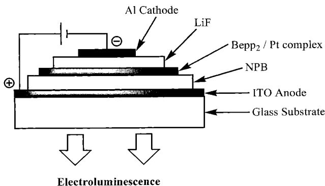
Schematic diagram of OLED in present invention
