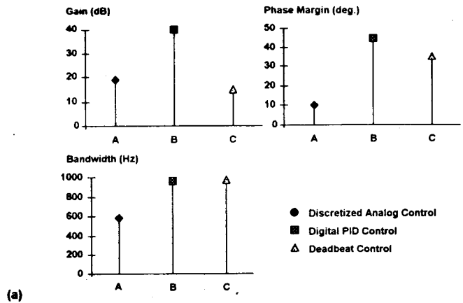
Fig. 8. Comparisons of experimental results of the three digital controllers
