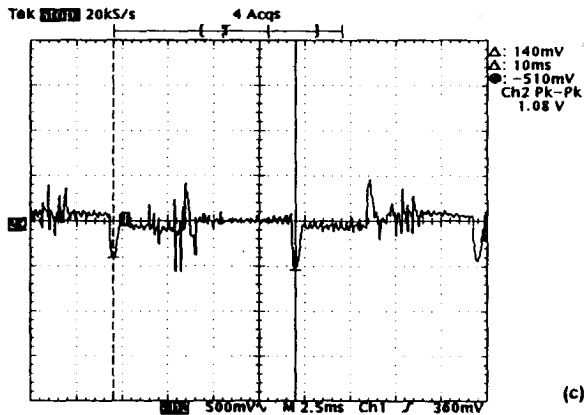
Fig. 9. Output voltage of (a) discretised analog controlled, (b) digital PID controlled, (c) deadbeat controlled power controllers
