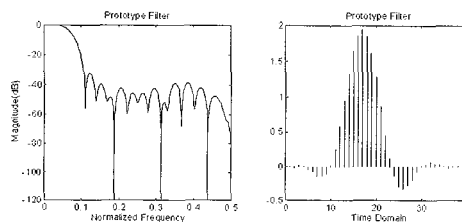
Fig.2 Prototype filter of 4-channel CMFB (a) Frequency response (b) Impulse response
