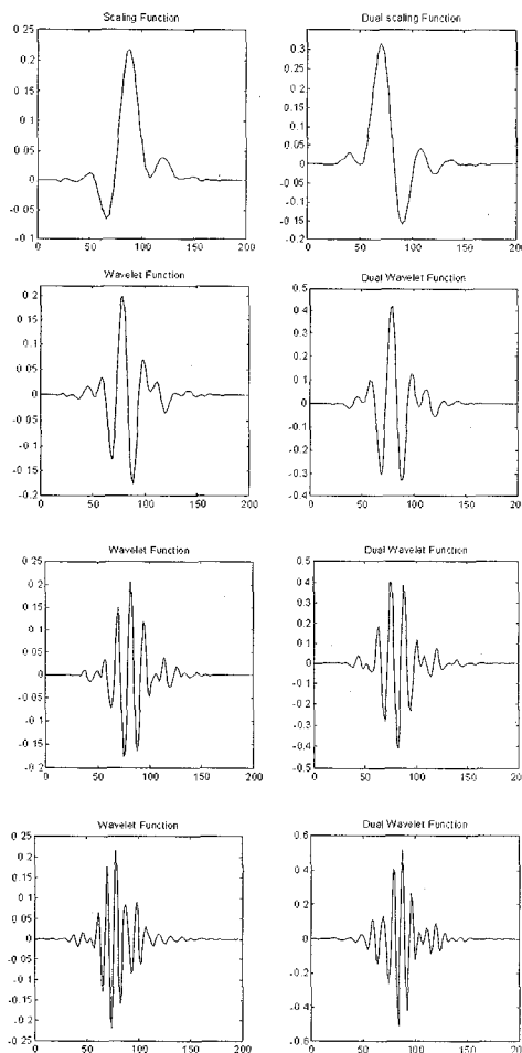
Fig.1 Scaling and wavelet functions and their dual functions
