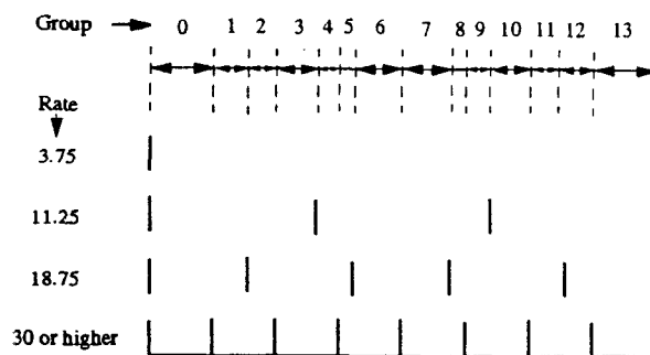
Figure 7: Macro-slots and groups in QuIVeR-1,2,3
