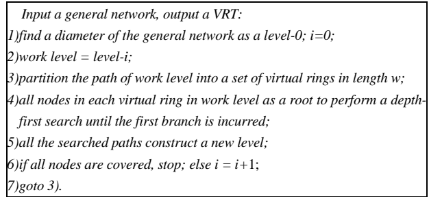
Figure 3.6 Algorithm of recursive construction of a VRT for general networks.
