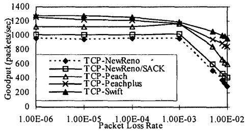
Fig. 5. Goodput performance comparison.
