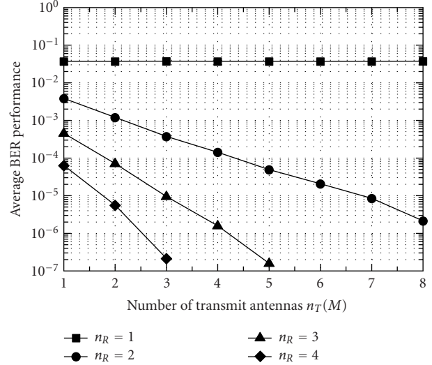
FIGURE 6: Average BER performance of the proposed iterative Pinv-MRC method with various number of users, n_T = M , and at SNR = 8 dB.
