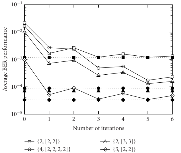
FIGURE 7: Average BER performance of the proposed iterative Pinv-MRC method for various number of iterations at SNR = 8 dB and 4-QAM.
